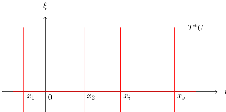
Figure 1 : \text{Car}(\widehat{\mathcal{D}}_{\mathfrak{x},k,\mathbb{Q}}^{(0)}/P) \cap T^*U
