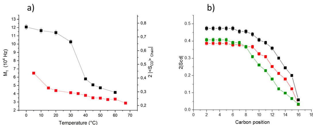
Fig. 7 Chain dynamics of DPPC, DoPhPC/DPPC, DoPhPC/DoPhPI/DPPC. (a) First spectral moment, M_1 , and corresponding whole chain ordering, 2S_{CD}^{chain} , (double y-axis) as a function of temperature for ^2\text{H}_{31} -DPPC (black squares) and DoPhPC/ ^2\text{H}_{31} -DPPC (red squares) water dispersions. 2S_{CD}^{chain} is the absolute value of chain ordering projected onto the bilayer normal and is 1 for rigid systems and 0 for liquids. 1 Accuracy is 2.5%. (b) Absolute value of carbon-deuterium order parameter, S_{CD}^k as a function of labelled carbon position, k , on the sn-2 DPPC chain, for ^2\text{H}_{31} -DPPC (black squares), DoPhPC/ ^2\text{H}_{31} -DPPC (red squares), DoPhPC/DoPhPI/ ^2\text{H}_{31} -DPPC (green squares), at 40 °C accuracy \pm 0.002 .
