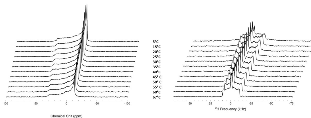
Figure S6. Left, ^{31}\text{P} -ssNMR spectra and right, ^2\text{H} -ssNMR spectra of a temperature run of water dispersions of DoPhPC + 20 mol% ^2\text{H}_{31} -DPPC. 20 minutes were waited after temperature equilibrium and before acquisition. Acquisition time at a given temperature is 42 min for ^{31}\text{P} -NMR and 34 min for ^2\text{H} -NMR representing a total time of 27hr for a full range of temperatures. Acquisition parameters were kept constant for all experiments and are given in materials and methods.
