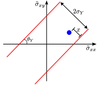
FIG. 11. A schematic plot of the yield surface for the tensorial model. The blue dot shows the state of a site in the shear stress space. The yield surface is described by two parallel lines separated by 2\sigma_Y and each line makes an angle of \theta_Y with \tilde{\sigma}_{xx} axis. The distance from the yield surface is shown by x .
