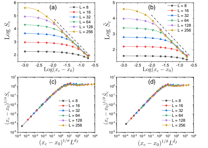
FIG. 18. Cut-off in avalanche distributions for the scalar model. (a, b): S_c = \langle S^3 \rangle / \langle S^2 \rangle (a) and \tilde{S}_c = \langle \tilde{S}^3 \rangle / \langle \tilde{S}^2 \rangle (b) versus x_c - x_0 for various system sizes. The dashed lines in (a) and (b) follow S_c \sim (x_c - x_0)^{-1/\sigma} and \tilde{S}_c \sim (x_c - x_0)^{-1/\tilde{\sigma}} , respectively. (c,d): Scaling collapse assuming Eq. (C4). The critical point x_c , exponents \sigma , \tilde{\sigma} , d_f , and \tilde{d}_f are determined by these scaling plots.
