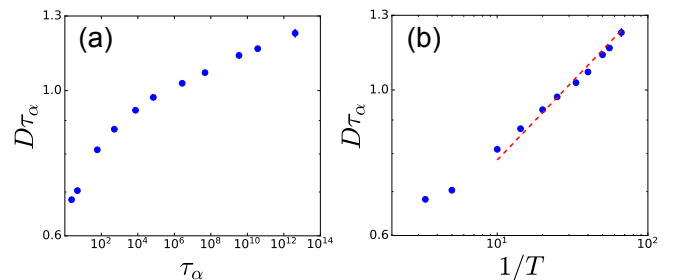
FIG. 10. The Stoke-Einstein decoupling D\tau_\alpha , where D is the diffusion coefficient of tracers, for the tensorial elasto-plastic model with L = 128 . (a): D\tau_\alpha versus \tau_\alpha could suggest an effective power-law behaviour (the fractional Stokes-Einstein violation), with two apparent exponents in the range \tau_\alpha < 10^4 and \tau_\alpha > 10^4 . (b): Our prediction suggests instead a power-law behaviour in terms of T . The red dashed line represents D\tau_\alpha \sim T^{-\nu(d_f - \bar{d}_f)} .
