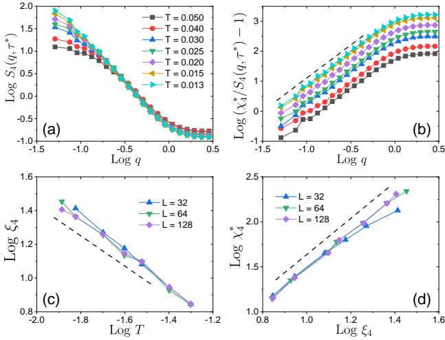
FIG. 13. The four-point structure factor S_4(q, t) and the associated correlation length \xi_4 for the scalar model. (a): S_4(q, \tau^*) for several temperatures for L = 128 . (b): The corresponding plot for the Ornstein-Zernike form in Eq. (B5). The dashed-line defines a slope corresponding to the exponent a . (c): The extracted \xi_4 versus T . The dashed line follows \xi_4 \sim T^{-\nu} . (d): \chi_4^* versus \xi_4 . The dashed line follows \chi_4^* \sim \xi_4^{d_f} .
