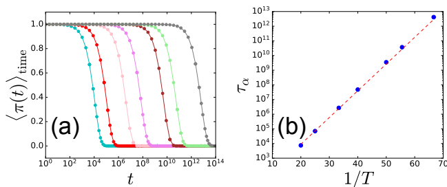
FIG. 1. Dynamics of the tensorial model in finite temperature simulations. (a): Mean persistence correlation function, \langle \pi(t) \rangle_{\text{time}} , for L = 128 and T = 0.050, 0.040, 0.030, 0.025, 0.020, 0.018, and 0.015 (from left to right). (b): The relaxation time \tau_\alpha versus 1/T . The red dashed-line corresponds to \tau_\alpha \sim e^{E_c/T} with E_c = x_c^{3/2} = 0.42 measured independently in Sec. IV.
