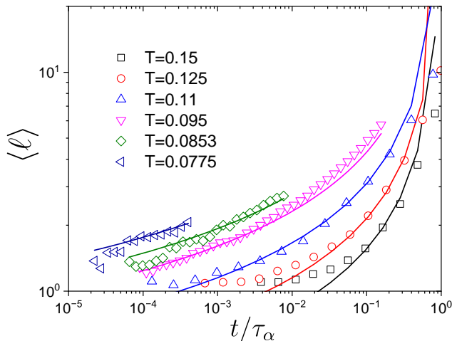
FIG. 8. Comparison between the molecular simulation data (empty points) in Ref. [51] and our theoretical prediction (solid curves) in Eq. (8) for the time evolution of a linear avalanche size \langle \ell \rangle . We set 1/\bar{\sigma} = 1.8 and \bar{d}_f = 2 , based on Table II. We use A = 0.6, 0.7, 0.9, 1.1, 1.2 and 1.3 for T = 0.15, 0.125, 0.11, 0.095, 0.0853 and 0.0775 , respectively.
