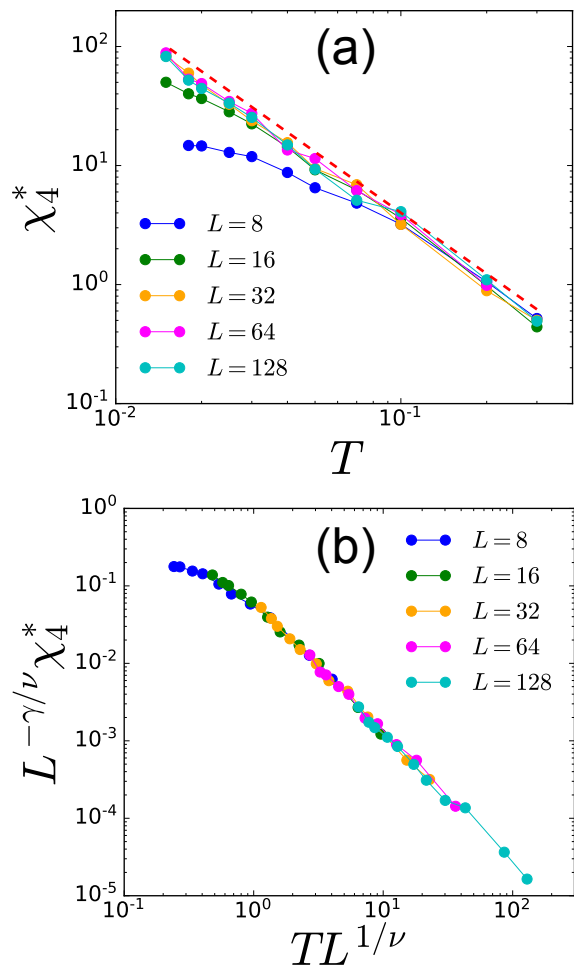
FIG. 3. (a): The peak of four-point correlation function, \chi_4^* , versus T for several L for the tensorial model. The red dashed-line follows \chi_4^* \sim T^{-\gamma} . (b): The corresponding scaling collapse.
