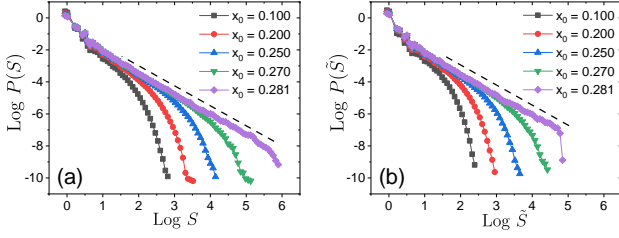
FIG. 17. Avalanche distributions P(S) (a) and P(\tilde{S}) (b) for several x_0 approaching the critical point x_c = x_0 = 0.281 for the scalar model with L = 256 . The dashed lines in (a) and (b) follow P(S) \sim S^{-\tau} and P(\tilde{S}) \sim \tilde{S}^{-\tilde{\tau}} , respectively.
