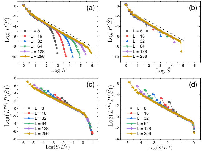
FIG. 19. (a,b): Distribution of avalanche size P(S) (a) and P(\tilde{S}) (b) for a stability threshold x_0 = x_c for the scalar model, with varying the system size L . The dashed lines follow P(S) \sim S^{-\tau} (a) and P(\tilde{S}) \sim \tilde{S}^{-\tilde{\tau}} (b). (c): The corresponding scaling collapse following Eq. (C2) with S_c \sim L^{d_f} . (d): Same for P(\tilde{S}) .
