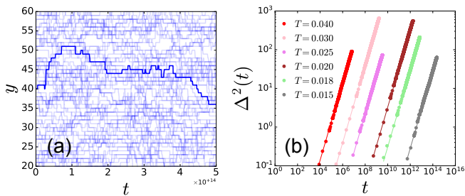
FIG. 15. Diffusion of tracer particles for the tensorial model with L = 128 . (a): The y component of typical trajectory of a tracer particle with T = 0.015 ( \tau_\alpha = 4.14 \times 10^{12} ). (b): Mean-squared displacement \Delta^2(t) of tracer particles are shown with points. The solid lines follow \Delta^2(t) = Dt , from which we extract the diffusion coefficient D .
