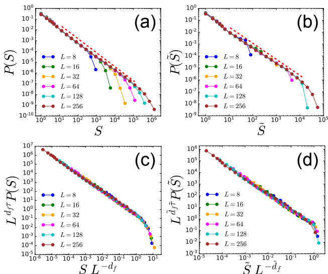
FIG. 6. (a, b): Distribution of avalanche size P(S) (a) and P(\tilde{S}) (b) for a stability threshold x_0 = x_c for the tensorial model, with varying the system size L . The dashed lines follow P(S) \sim S^{-\tau} (a) and P(\tilde{S}) \sim \tilde{S}^{-\tilde{\tau}} (b). (c, d): The corresponding scaling collapse following Eq. (2) with S_c \sim L^{d_f} (c). The same expressions are used for P(\tilde{S}) in (d).
