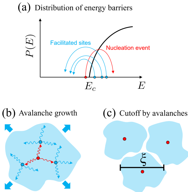
FIG. 9. Proposed picture for dynamical heterogeneities in glass-forming liquids. (a): At low temperatures, the distribution of activation energy barriers P(E) presents a gap below some energy E_c . On a time scale \tau_\alpha \sim e^{E_c/T} , a site with a barrier near E_c relaxes (red arrow), which we call a "nucleation event". As a result, due to elastic interactions, other sites may display lower barriers E < E_c (blue arrows), which we call "facilitated sites". They relax on a time scale much faster than \tau_\alpha , leading to a rapid sequence of events, forming a thermal avalanche. The corresponding real space picture is shown in (b, c). (b): A nucleation event (red circle) triggers facilitated sites (blue circles) by elastic interactions (wavy arrows). These induced events again induce other sites, forming an avalanche growth. (c): Avalanche growth is cut off due to other avalanches originating from different nucleation events taking place simultaneously in the system. The cutoff length \xi corresponds to the maximum size for which extremal dynamics applies, which defines the length of dynamical heterogeneity at finite temperature.
