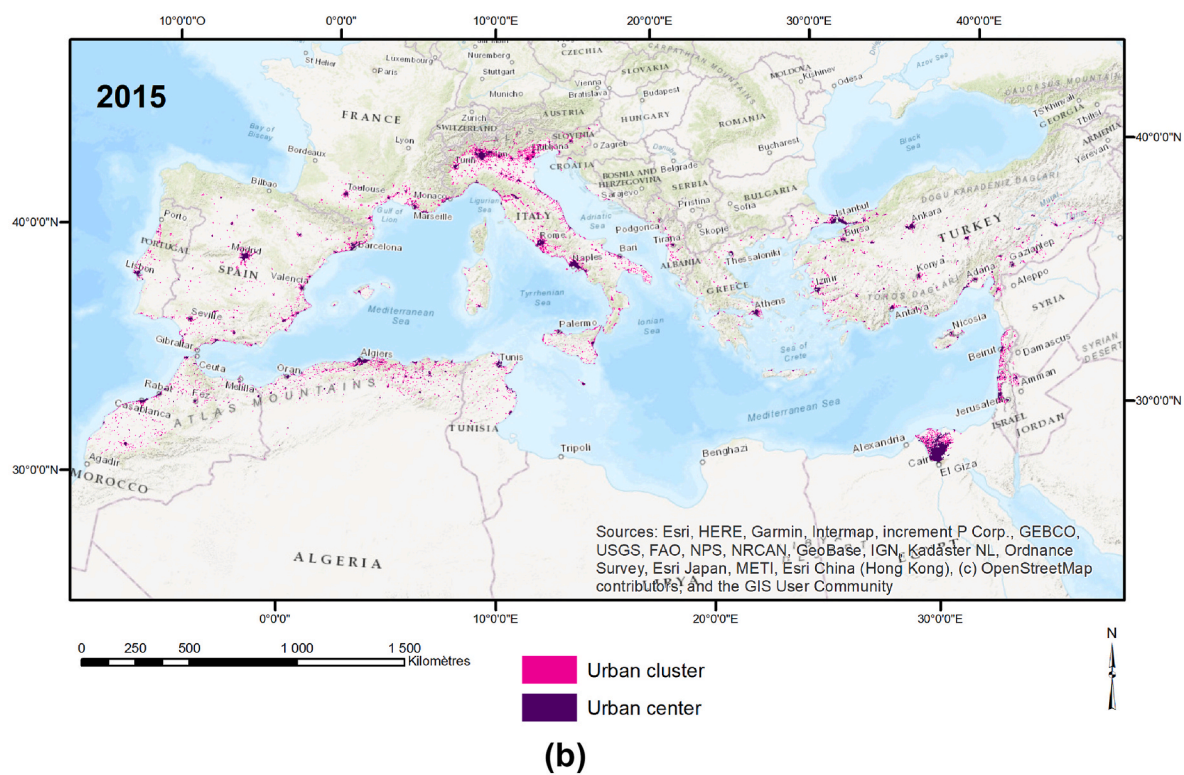
Fig. 3. a Clusters of high increase in farming intensification, concentration and/or specialisation of food production in 2015. Fig. 3b. Urban clusters and urban centres in 2015. Source: Global Human Settlement Layer.
