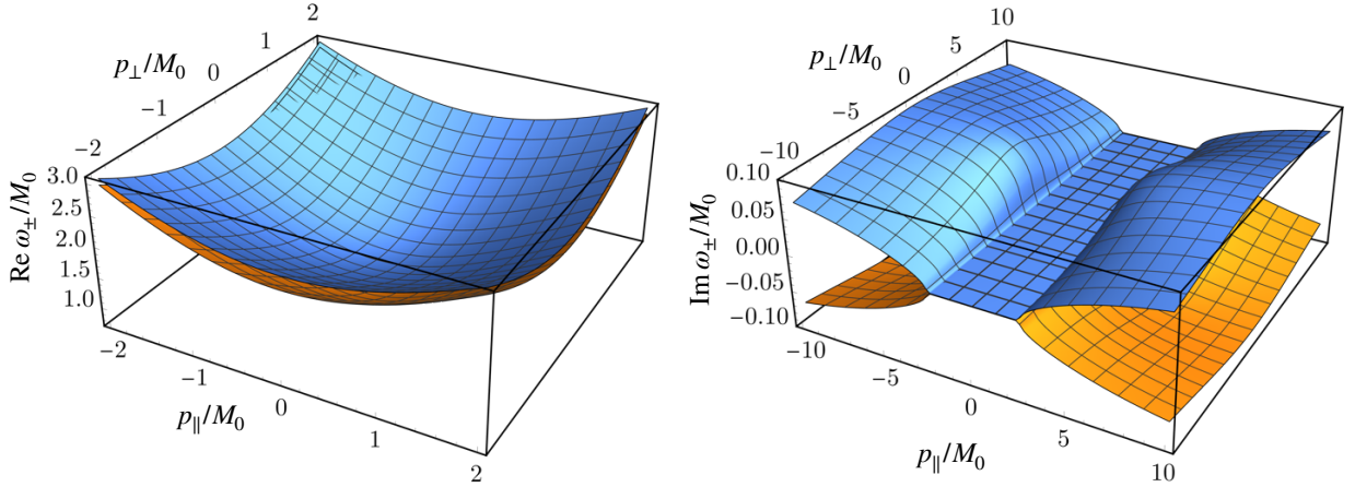
FIG. 6. The real (left) and imaginary (right) parts of the energy dispersions \omega_{\pm} for the spacelike similarity field C^{\mu} \equiv (0, 0, 0, C_3) \neq 0 for the same set of parameters as in Fig. 6. The imaginary parts develop when the longitudinal momentum p_{\parallel} \equiv p_3 exceeds the critical momentum p_{\max}^{(s)} [see Eq. (119)]. The plots are shown in the (p_{\parallel}, p_{\perp}) plane, where p_{\perp} = \pm\sqrt{p_1^2 + p_2^2} is the transverse momentum.
