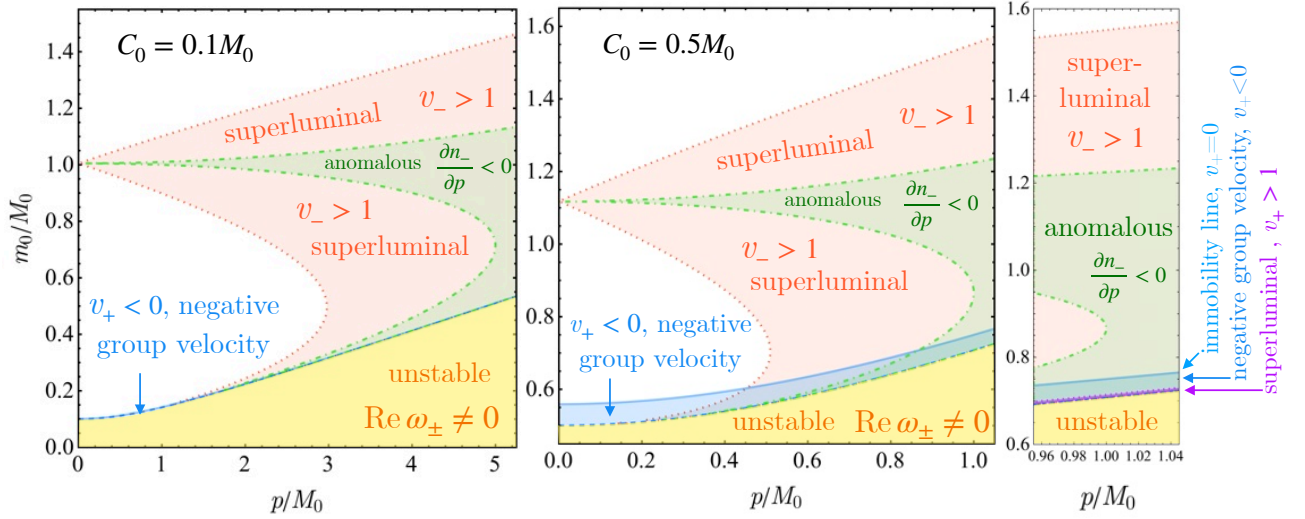
FIG. 5. The regions in the (p, m_0) plane at C_0 = 0.1M_0 (left) and C_0 = 0.5M_5 (middle) of: the high-momentum instability (yellow for both modes), superluminal propagation (red for “-”-mode and magenta for “+”-mode), anomalous dispersion of the “-”-mode (green), the line of immobility of the “+”-mode (blue), and the negative group velocity of the “+”-mode (blue). A zoom-in on a region around p = M_0 for C_0 = 0.5M_5 (right) also shows the region where the “+”-mode becomes superluminal with negative group velocity (magenta). The blue and yellow regions are separated by the critical momentum (110).
