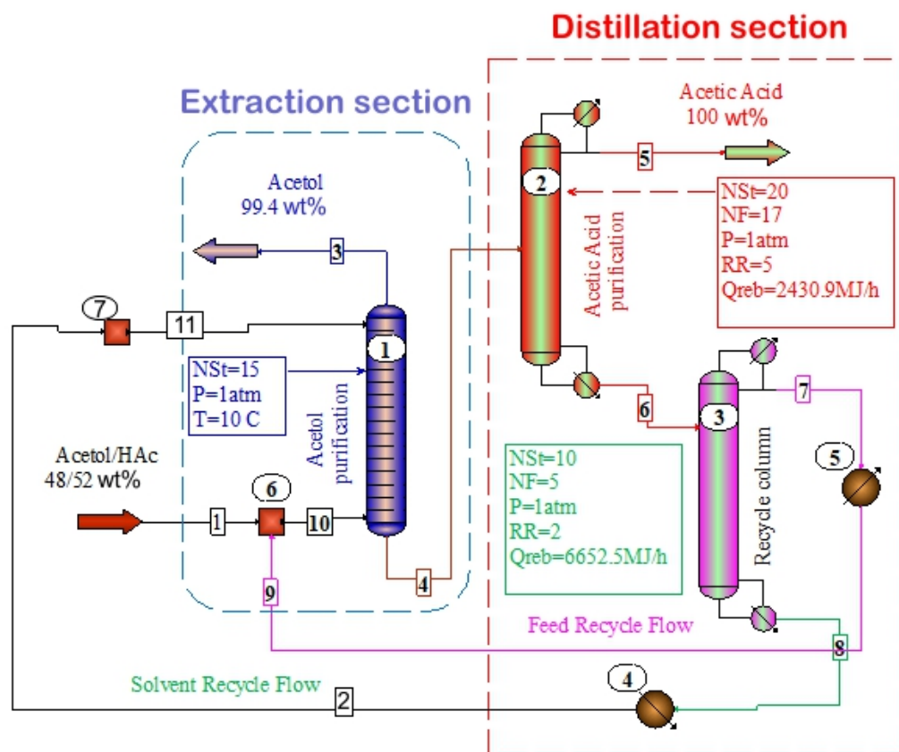
Figure 2. Flowsheet for A/HAc separation.
