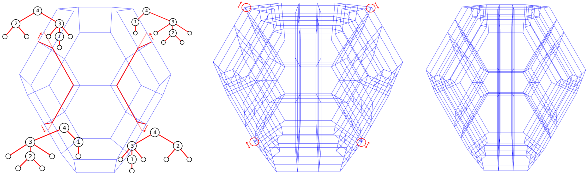
FIGURE 28. Construction of a 3 dimensional realization.
