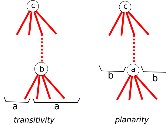
FIGURE 6. Illustration of the transitivity and planarity conditions on s -tree inversion sets. (Figure 5 of [CP22])
