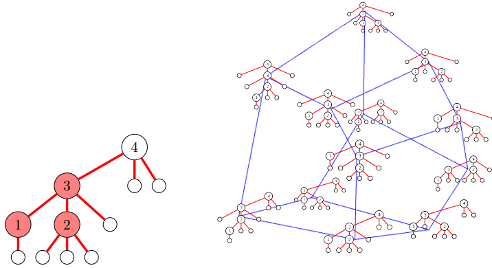
FIGURE 11. Example of a pure interval. the minimal tree of the interval with selected tree-ascents and on the right, the interval drawn as the skeleton of a 3d polytope.
