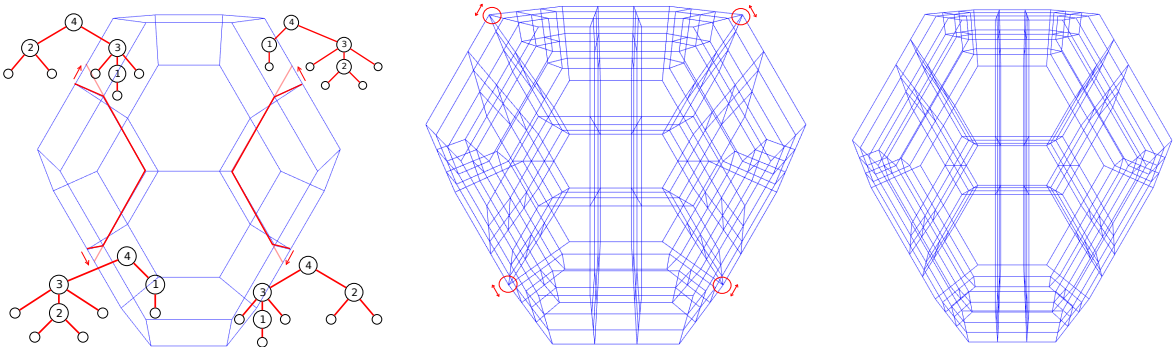
FIGURE 28. Construction of a 3 dimensional realization.
