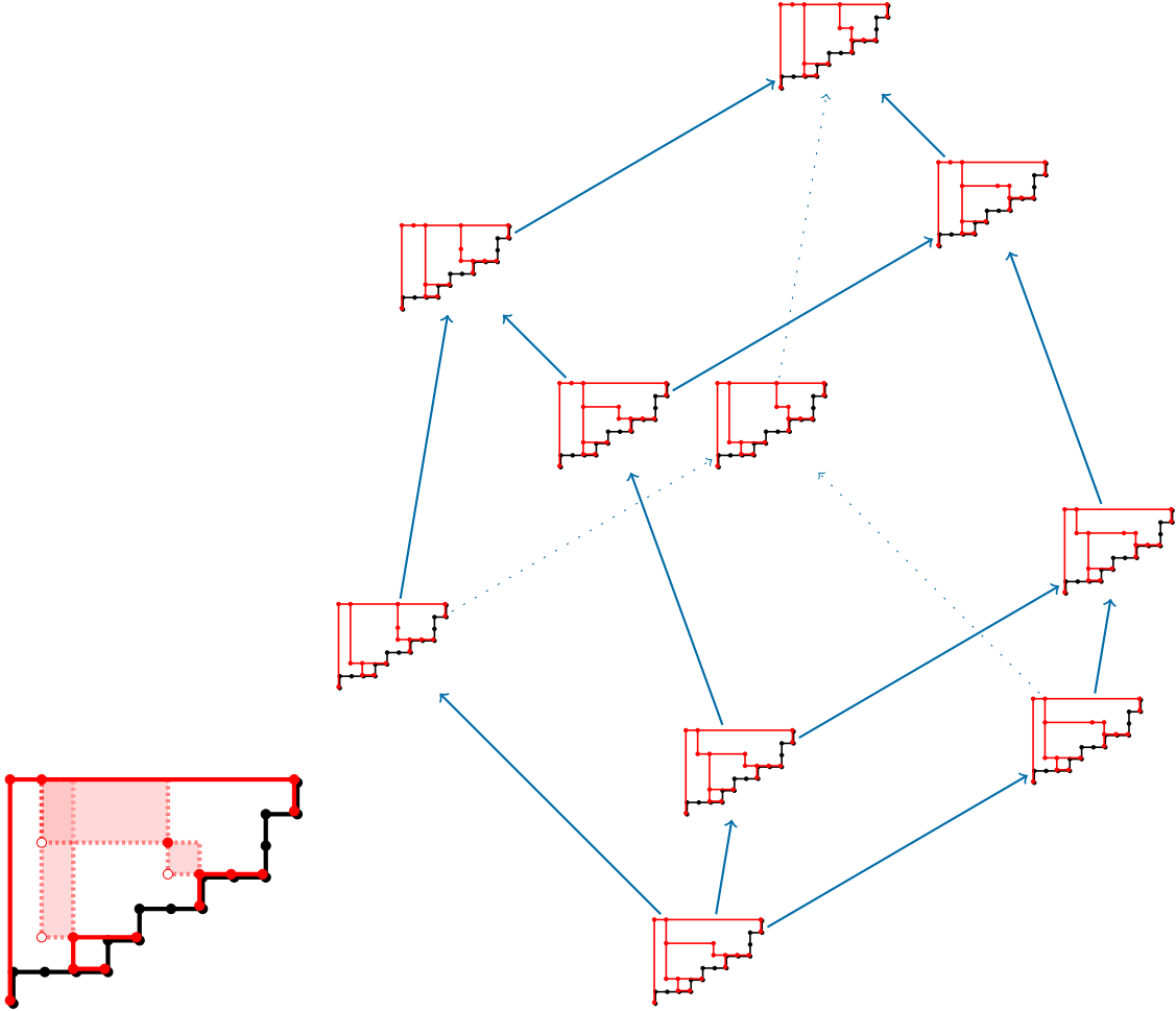
FIGURE 21. Example of a pure \nu -Tamari interval
