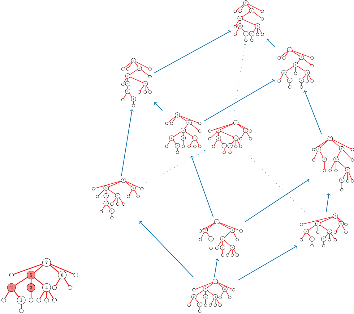
FIGURE 19. Example of a 3-dimensional pure s -Tamari interval.
