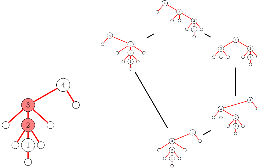
FIGURE 9. Example of a pure interval. On the left, the minimal tree with colored tree-ascents and on the right the corresponding interval.
