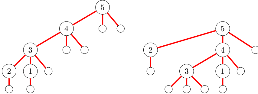
FIGURE 14. A +1-interval that is not a pure interval.
