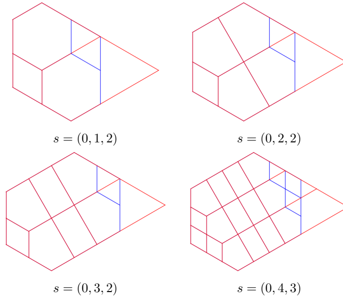
FIGURE 24. Realizations of s -associahedra from s -permutahedra
