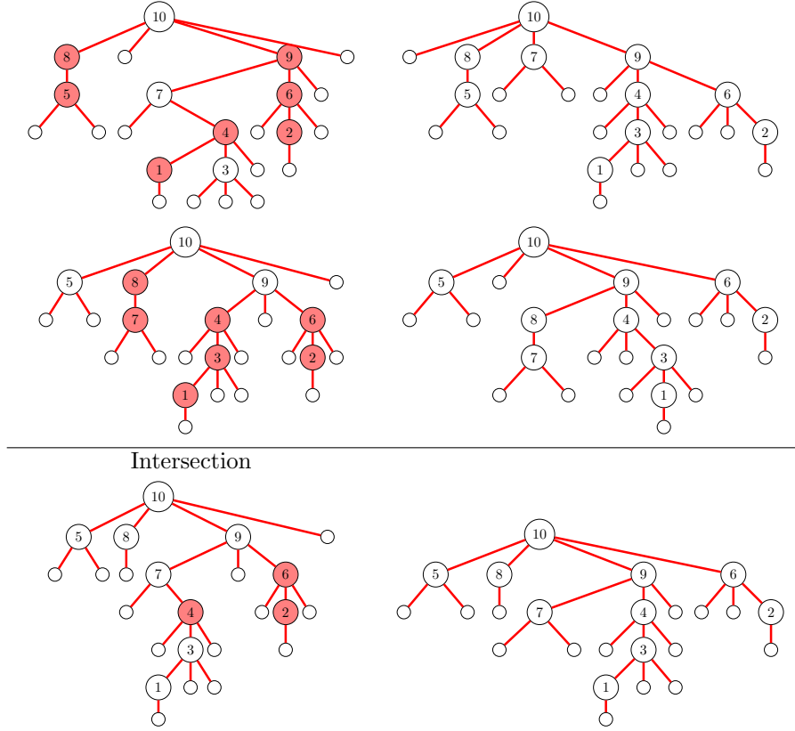
FIGURE 16. Example of an intersection of pure intervals in size 10
