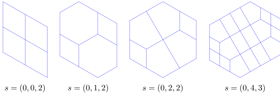
FIGURE 22. Some geometric realizations of s -permutahedra in dimension 2.
