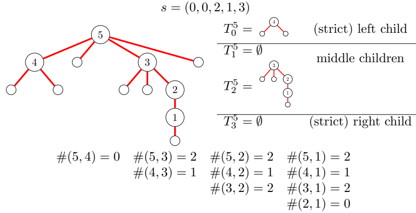
FIGURE 5. an s -decreasing tree and its tree-inversions (Figure 4 of [CP22])
