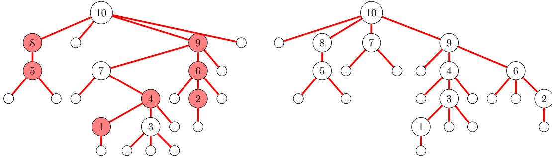
FIGURE 10. Example of a pure interval. On the left, the minimal tree of the interval with selected tree-ascents and on the right, the maximal tree of the corresponding interval.
