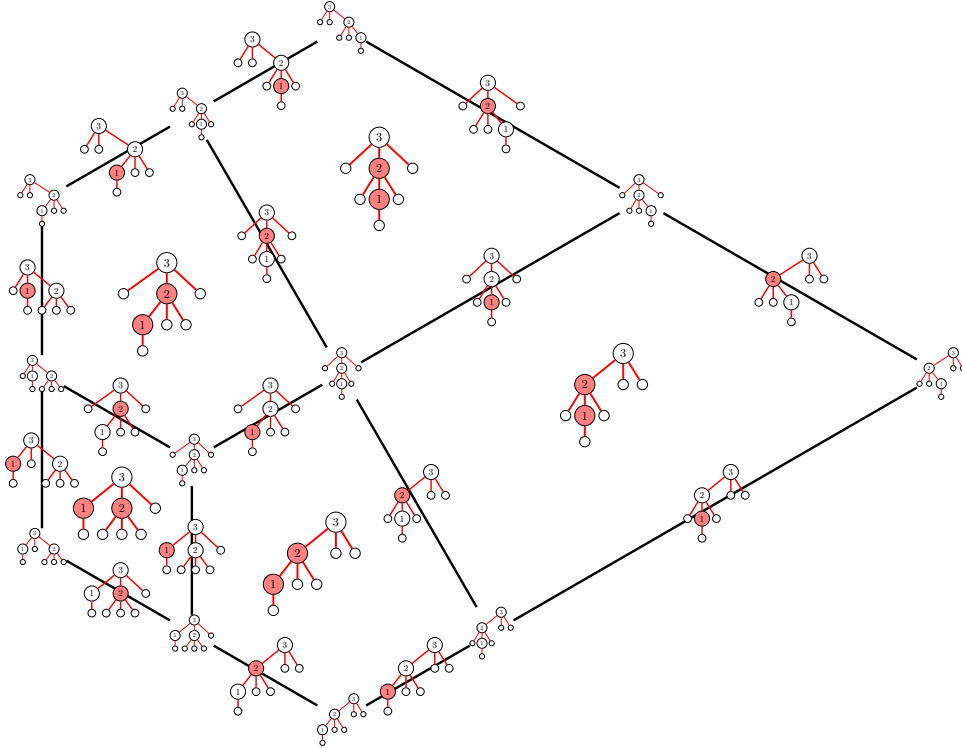
FIGURE 3. The s -Tamari lattice as the edge graph of the s -associatedhedron for s = (0, 2, 2)
