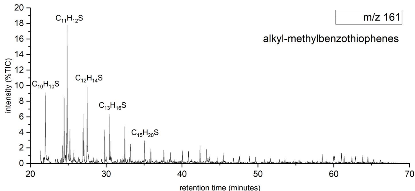
Fig. S5. GC-MS of the bitumen of Orbagnoux sample DP, selected mass chromatograms. Both m/z 57 and 55 are dominated by alkane fragments. The peaks at m/z 125 comprise a series of n -alkyl-ethylthiophenes (indicated by C y , with y = total C number), and a series of isoprenoid alkylthiophenes (indicated by iC y ) including the base peak assigned to 2,3-dimethyl-5-(2,6,10-trimethylundecyl)thiophene (iC 20 H 36 S), and isoprenoid thiophene with a phytane skeleton that has also been identified in Orbagnoux by van Kaam-Peters and Sinninghe Damsté (1997). The signal at m/z 139 is dominated by alkyl-propylthiophenes. That at m/z 161 is dominated by alkyl-methylbenzothiophenes. Note that the most intense peak of the ion chromatogram at m/z 97 (not shown) had an intensity (relative to TIC) of 1.25%, showing the low abundance of alkylthiophenes relative to the alkyl-methylthiophenes.
