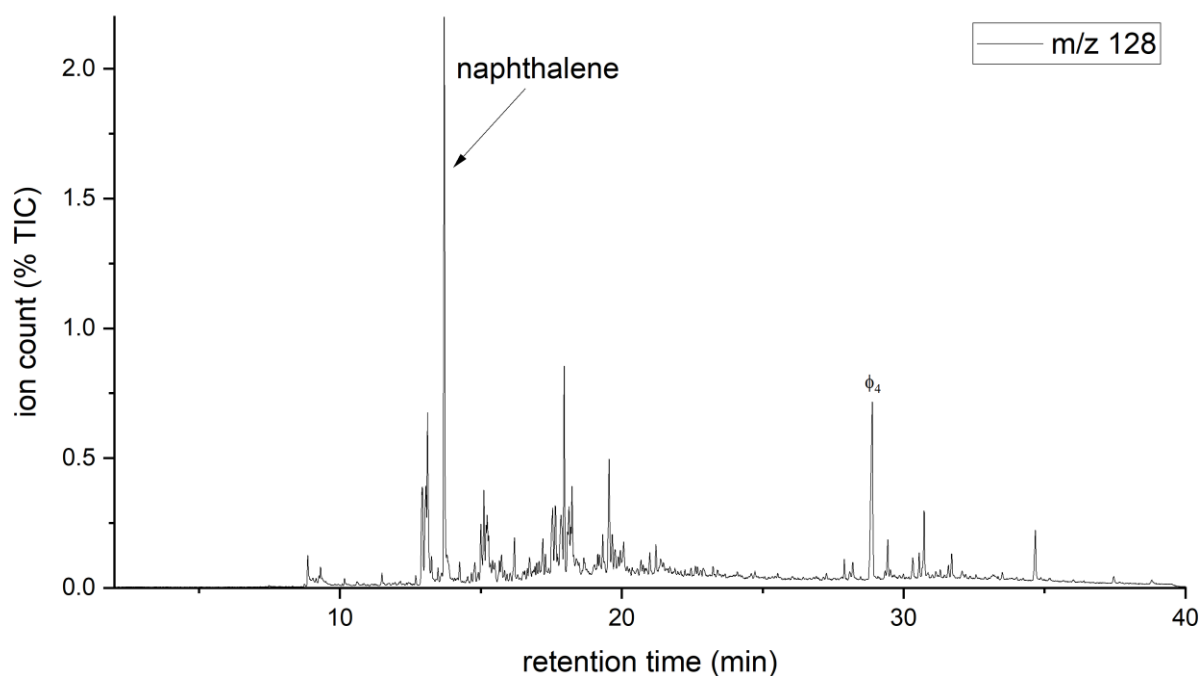
Fig. S12. Orbagnoux kerogen, 600°C pyrolysis GC-MS, selected ion mass chromatogram, m/z 128, dominated by the contribution of naphthalene.
