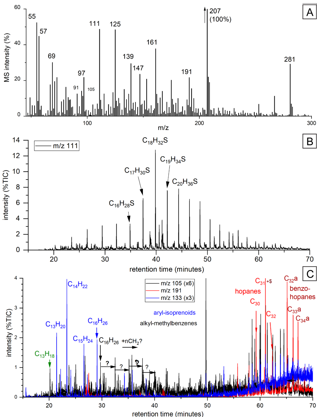
Fig. 6. GC-MS of the bitumen of Orbagnoux sample DP. (A) Total GC-MS mass spectrum obtained by integrating all mass spectra for all retention times. The signals at m/z 207 and 281 are dominated by column bleed. (B) Mass chromatogram of m/z 111 showing series of alkyl-methylthiophenes. (C) Mass chromatograms of m/z 105, 133 and 191 showing alkylated aromatics including benzohopanes, alkyl-methylbenzenes and benzohopanes, as well as
