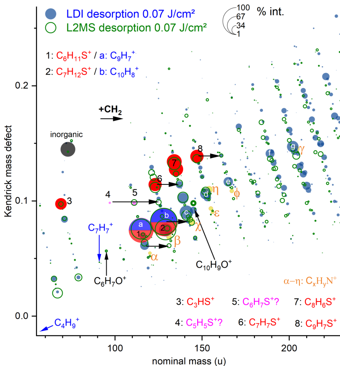
Fig. 7. ORBA3 kerogen analyzed with L2MS and LDI-MS , in positive polarity, using desorption at 266 nm. Mass defect plot from positive polarity spectra recorded in LDI-MS and L2MS, with 0.07 J/cm 2 fluence for desorption, and 0.08 J/cm 2 fluence for ionization at 266 nm in L2MS. See Figs. S2C and S3F-G for full spectra. L2MS peaks shown in open green circles. In the LDI-MS spectrum, species identified as sulfurated molecules are shown in red, peaks with likely interference of hydrocarbons and sulfurated molecules are shown in blue/red combination disks, peaks assigned to C x H y N + in yellow (α-η), and other peaks without isotope support to assignments are shown in dark blue. Peaks 4, 5 (pink) are tentatively attributed to sulfurated fragments. Peaks (a-g) are attributed to PAHs (see main text).
