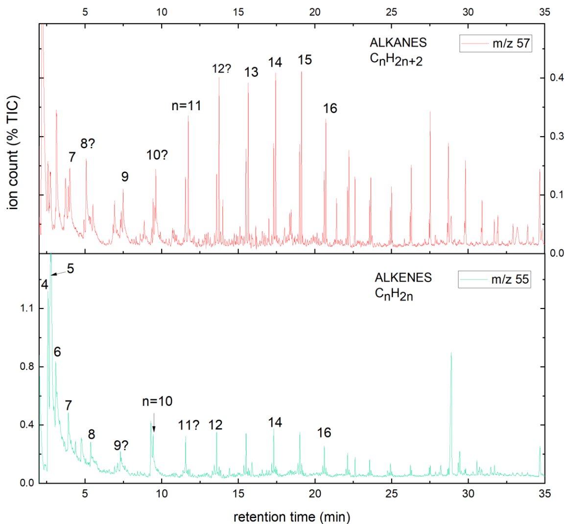
Fig. S10. Orbagnoux kerogen, 600°C pyrolysis GC-MS, selected ion mass chromatograms. The mass chromatograms at m/z 57 and m/z 55 are dominated by n -alkanes and n -alkenes, respectively ( n values shown with each peak).
