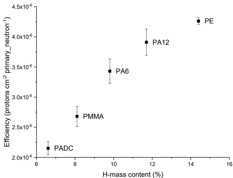
Fig. 9. Conversion efficiencies of several materials, typically used as converters, as function of the hydrogen mass content in the material composition. Reproduced from Stabilini (2021).
