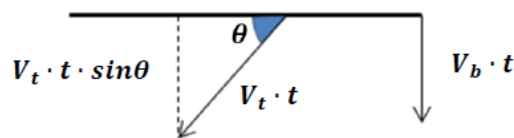
Fig. 4. Sketch for the demonstration of the critical angle formula (assuming a constant V_t ). The horizontal line refers to the PADC height just before the etching of the latent tracks begins.
