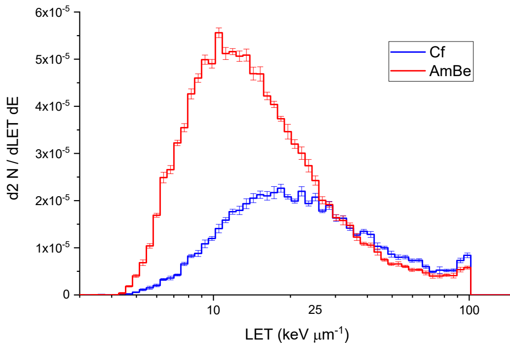
Fig. 6. Recoil protons versus LET in water generated by neutrons interacting with a 2 mm PMMA converter simulated for the neutron spectrum 241 AmBe and 252 Cf sources using the FLUKA code. Reproduced from Stabilini (2021).
