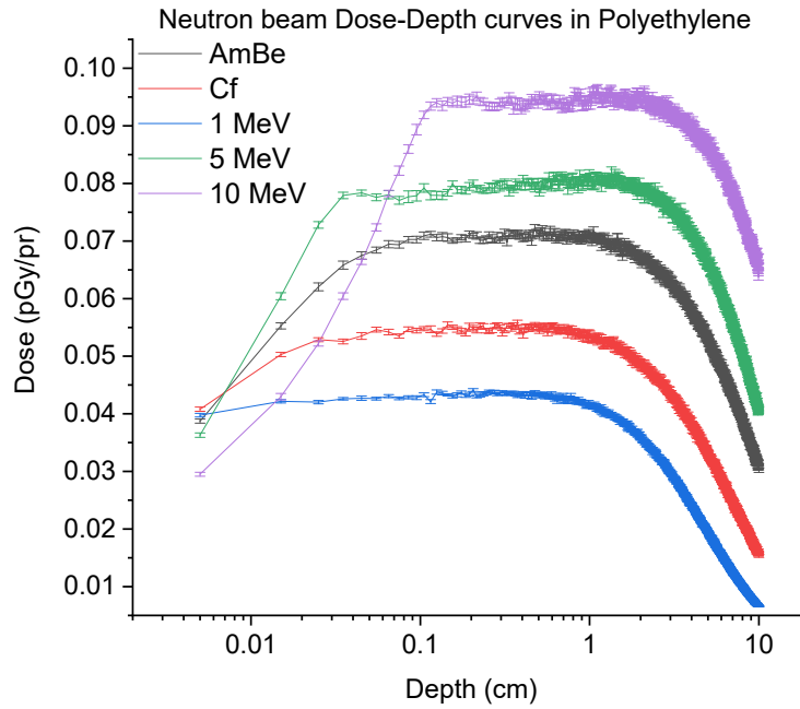
Fig. 8. Dose-depth curves in polyethylene for mono-energetic neutron beams with different energies, as well as for the neutron spectrum from ^{241}\text{AmBe} and ^{252}\text{Cf} sources, simulated using the FLUKA code. Reproduced from Stabilini (2021).
