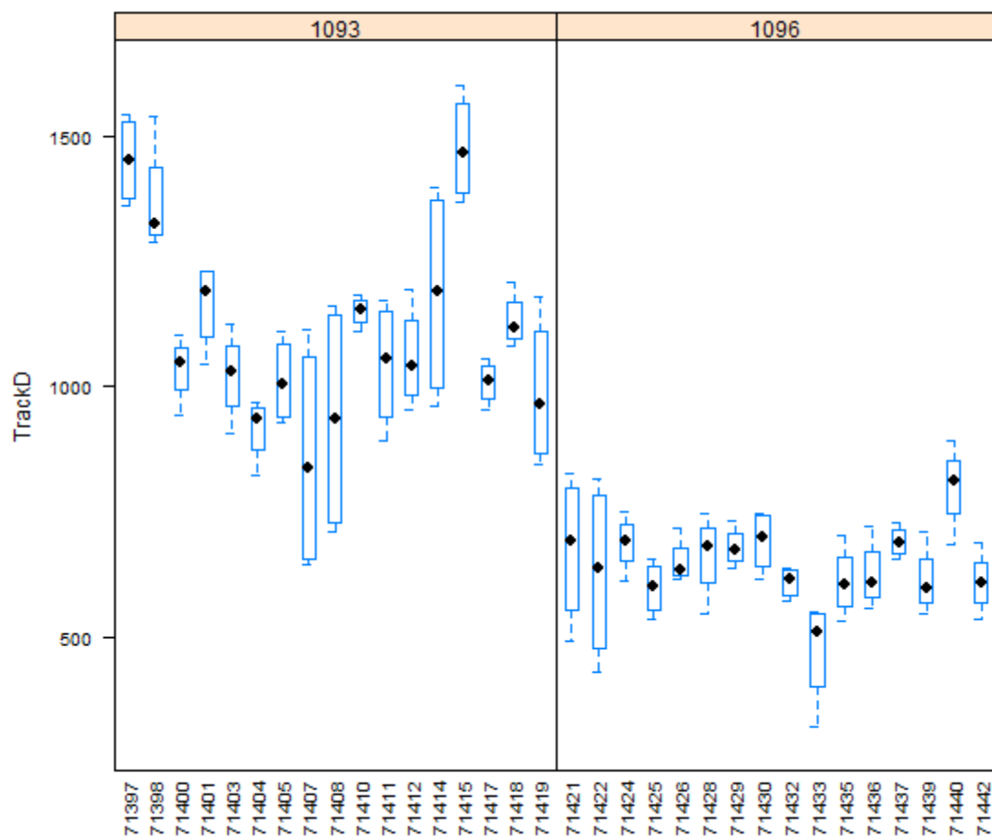
Fig. 12. Example of acceptance test results (track density in tracks \text{cm}^{-2} ) for (a) unirradiated detector and (b) irradiated detectors for various batches (four-digit number) and sheets (five-digit numbers).
