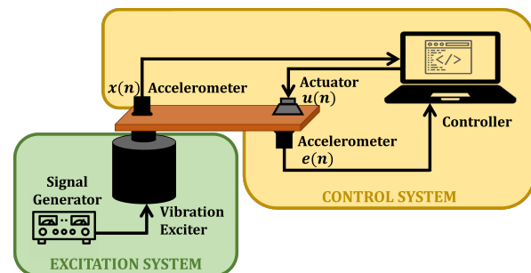
Figure 3. Drawing of the test bench used during experiments.
