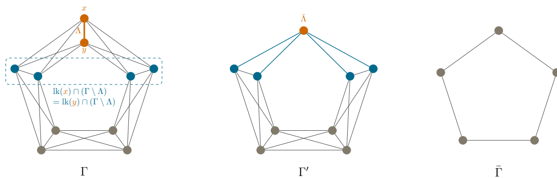
Figure 11: Collapsible and strongly reduced graphs (Example 6.2)
