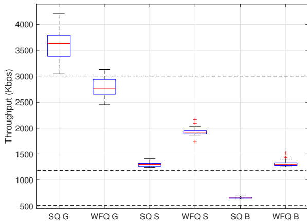
Figure 5: sLB and SQ vs sLB and WFQ: throughput results. The removal of SQ leads to violations in gold flows’ throughput results.
