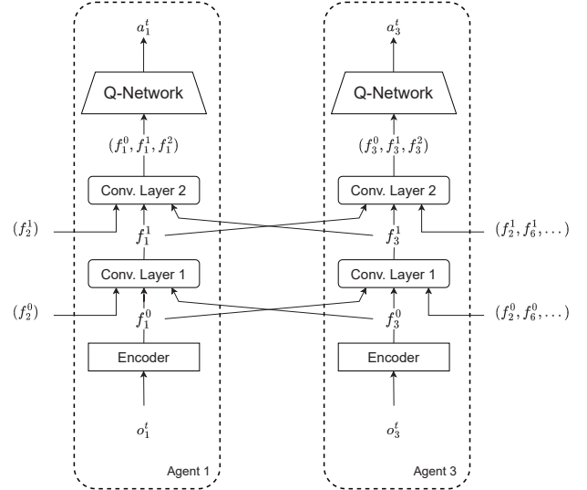
Figure 3: Structure of two communicating DGN agents
