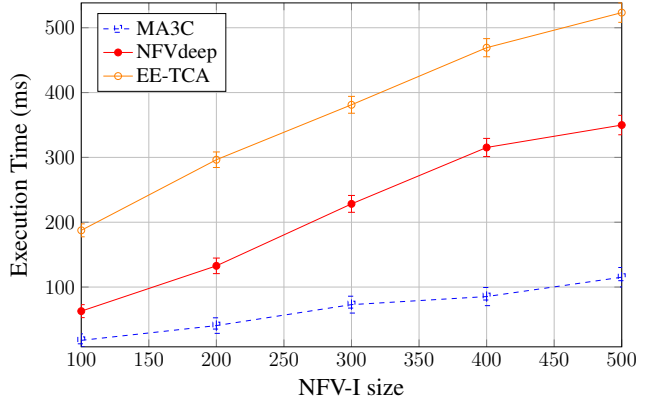
Fig. 5: Execution Time w.r.t NFV-I size variation (NFV-I size = up to 500, VNF-FG size = 5).
