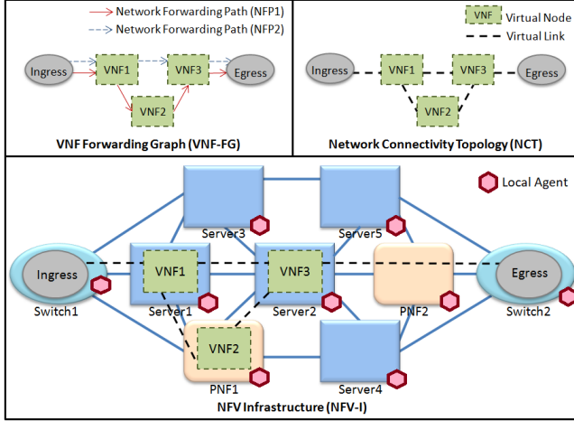
Fig. 1: Mapping of the VNF-FG in the NFV-I.
