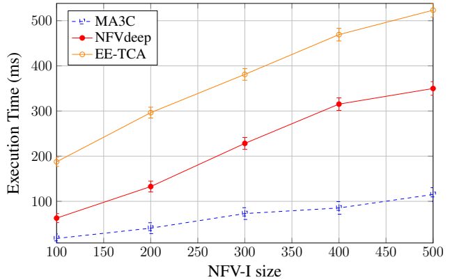
Fig. 5: Execution Time w.r.t NFV-I size variation (NFV-I size = up to 500, VNF-FG size = 5).
