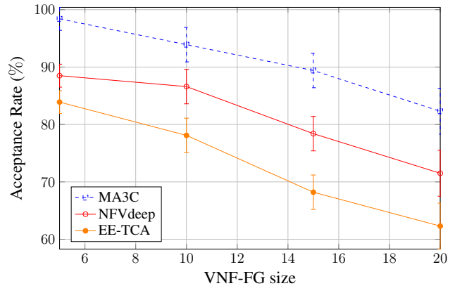
Fig. 4: Acceptance percentage w.r.t VNF-FG size variation (NFV-I size = 200, VNF-FG size = up to 20).
