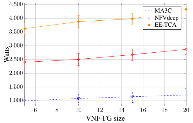
Fig. 3: Power consumption w.r.t VNF-FG size variation (NFV-I size = 200, VNF-FG size = up to 20).
