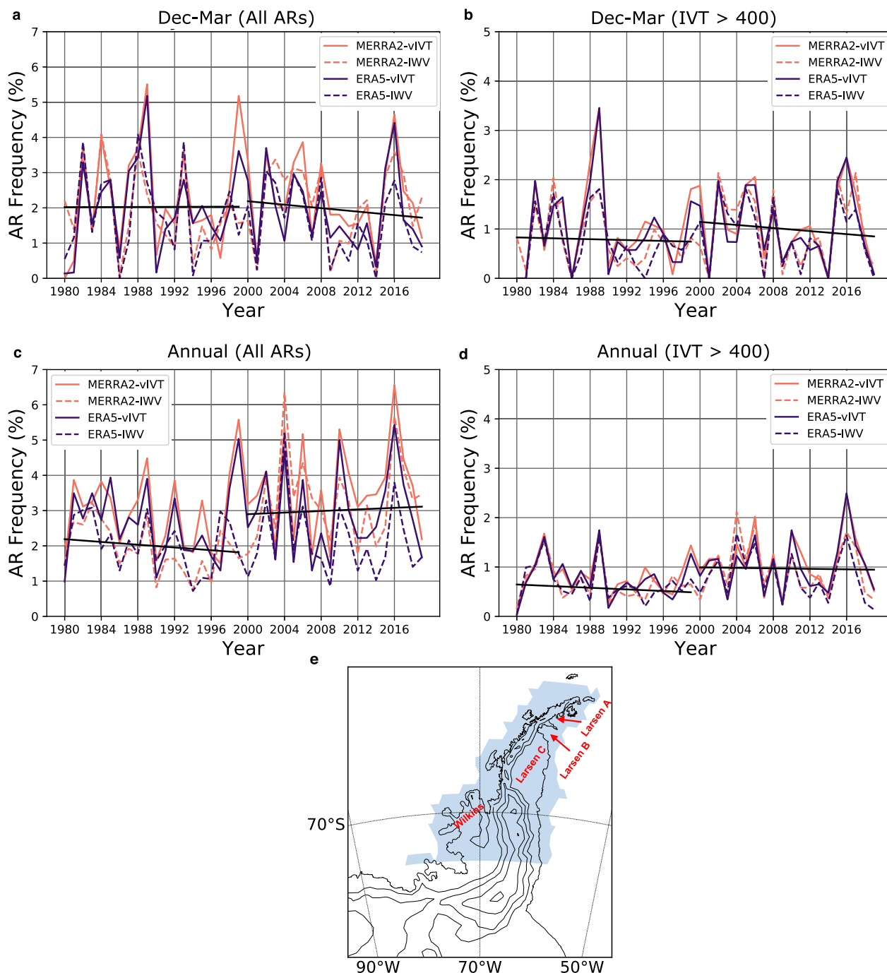
Fig. 1 Annual AR frequency and trends. Frequency of AR landfalls on the Antarctica Peninsula for a, b December–March and c, d yearly according to the vIWT and IWV AR detections schemes when applied to MERRA-2 and ERA-5 reanalysis. b, d represent the AR frequency when all AR landfalls with a maximum IVT below 400 \text{ kg m}^{-1} \text{ s}^{-1} are removed from the record. The year in a and b refers to the austral summer of December, January, February, March (i.e., the austral summer of 1988–1989 is referenced as 1989 in the plots). An AR landfall is counted if an AR shape touches the region highlighted in e which also shows the locations of the Larsen A and B embayments, Larsen C ice shelf, and Wilkins ice shelf.
