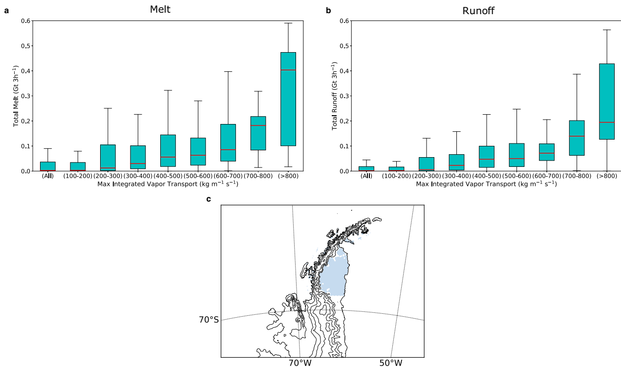
Fig. 5 The relationship between AR intensity and melt/runoff intensity. The maximum integrated vapor transport (IVT) upon landfall for each detected AR timestep and the corresponding 3-hourly cumulative a surface melt and b runoff over c the area shaded in blue using MERRA-2 for IVT and MAR for surface melt and runoff. The most common IVT intensity was 300–400 kg m -1 s -1 ( n = 273 ), while the least common IVT intensity was >800 kg m -1 s -1 ( n = 14 ) over the December–March period. The boxes represent values from the first to the third quartile, the red line is the median, and the whiskers extend to the data maximum and minimum. The area of the blue shaded region is ~91,400 km 2 .
