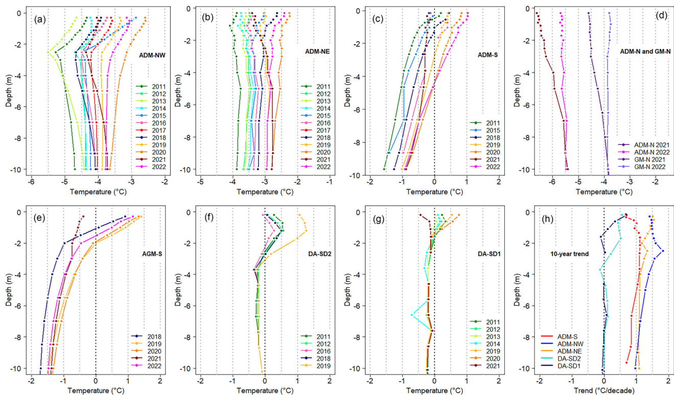
FIGURE 11 (a–g) Mean annual temperature–depth (Tz) profiles; (h) linear trend calculated with the annual values along Tz profiles for the reference decade 2011–2020.
