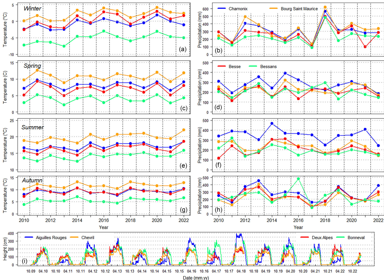
FIGURE 4 Seasonal air temperature (a, c, e, g) and precipitation (b, d, f, h), as well as daily maximum snow height at the different weather stations (i).
