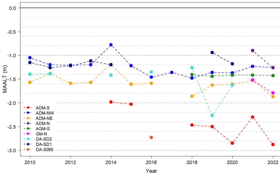
FIGURE 9 Mean annual active layer thickness (MAALT) for the available years.
