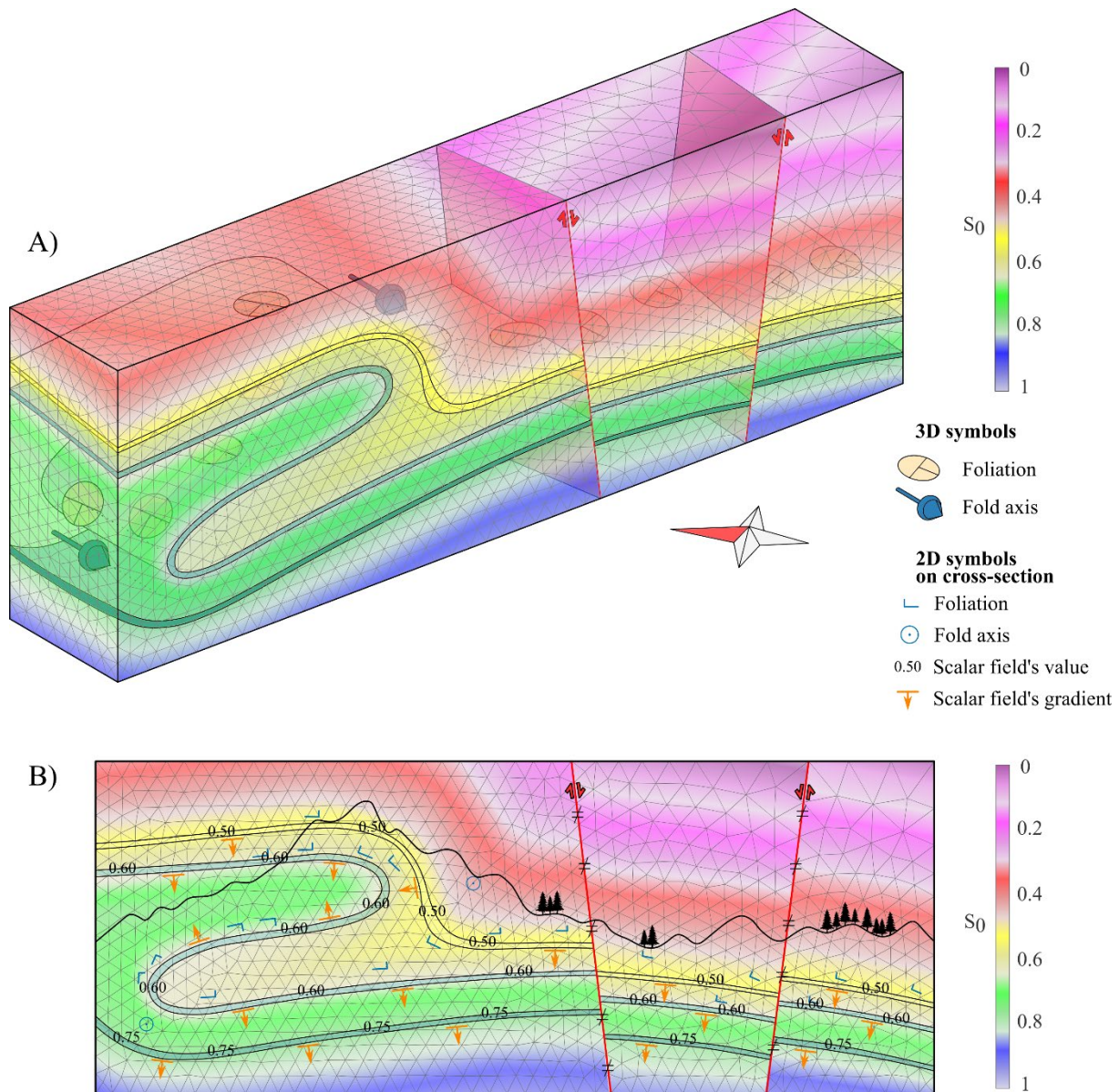
Figure 8. (A) 3D and (B) cross-section views of the synthetic scenario in Fig. 6 displaying isoclinal recumbent folding and normal faulting. The implicit approach is employed to interpolate the 3D structural model, using geological and structural data as value and gradient constraints.
