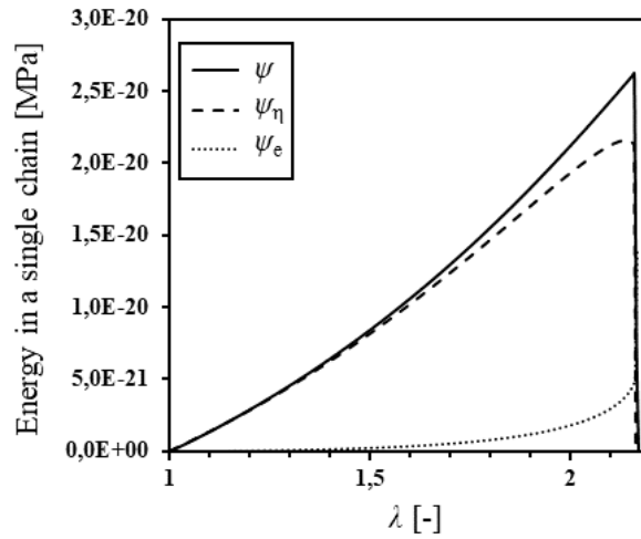
Fig. 4 Evolution of the total strain energy density \psi , of the entropic. contribution \psi_\eta , and of the bond energy \psi_e of a single chain as a function of the total stretch \lambda . The parameter values used for generating these results are the following: n=4.5 \cdot 10^{20} \text{ cm}^{-3} , N=10 , e/k.T=3.44 , \alpha_1=9 , \alpha_2=5\alpha_1
