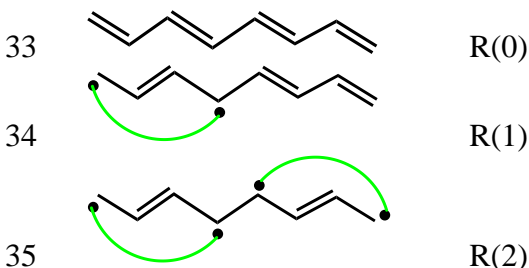
36 Scheme 4: Structure labeling [3], in R(i), i counts the couple of unpaired electrons.
