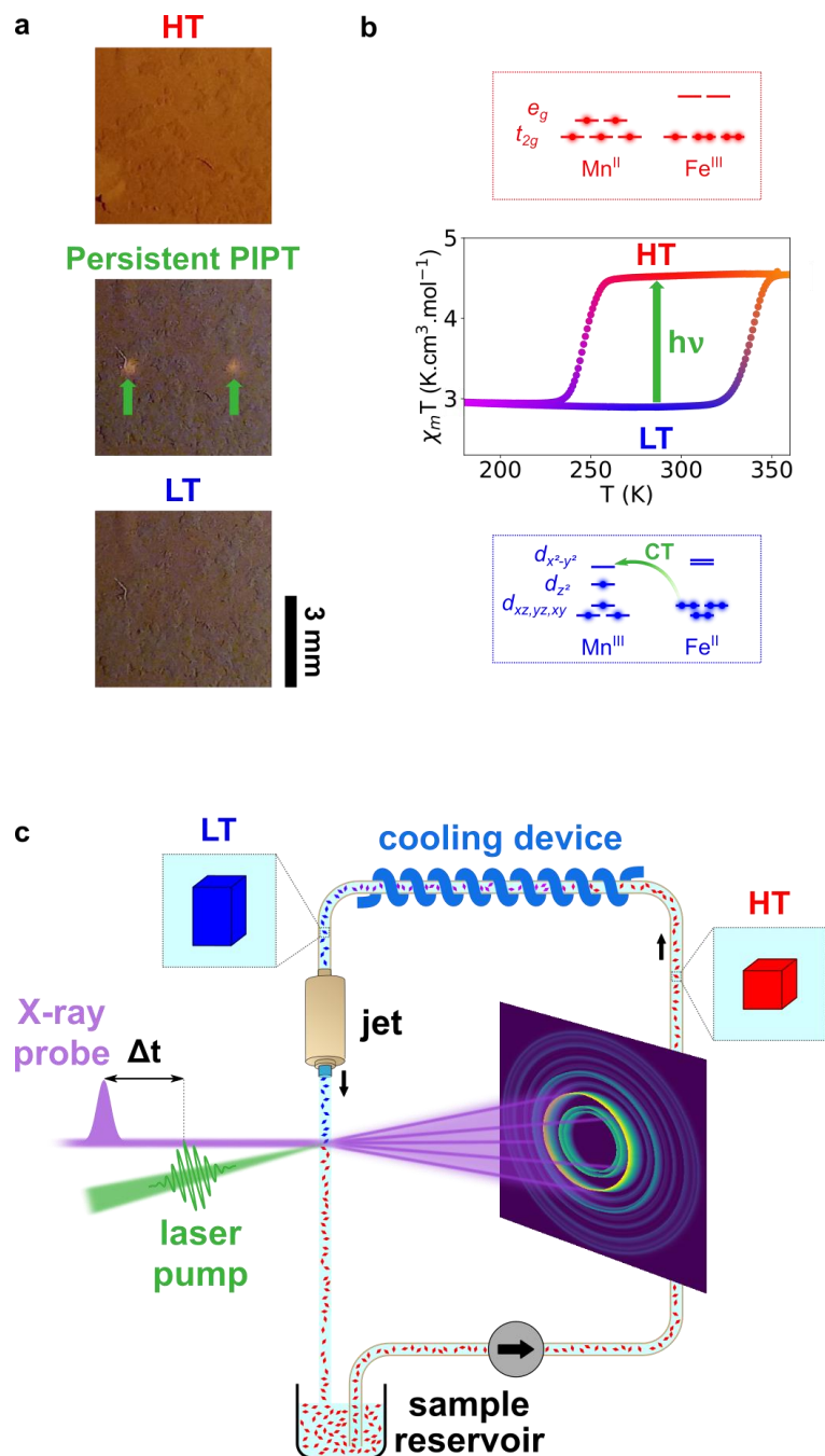
Figure 1. Charge-transfer bistability at room temperature. a Pictures of 6×6 mm 2 RbMn 0.94 Co 0.06 Fe thin films taken at room temperature, showing the colour change between the Mn III (S=2)Fe II (S=0) low-temperature (LT) and Mn II (S=5/2)Fe III (S=1/2) high-temperature (HT) phases. Starting from the LT phase, a persistent photoinduced phase transition (PIPT) is induced by laser excitation (120 W.cm -2 , 0.2 mm 2 spot size, 3 s irradiation), as characterized through colour change at laser spots positions (green arrows). Subsequent heating of the irradiated film yields global colour change over the whole film in the HT phase. b Thermal hysteresis between the HT and LT phases,
