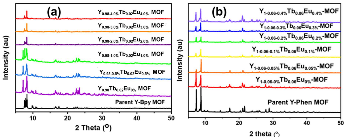
Figure S2. PXRD patterns of (a) Y_{0.98-x}Tb_{0.02}Eu_{x\%} -MOF samples (bpy series) and (b) Y_{1-0.06-x}Tb_{0.06}Eu_{x\%} -MOF samples (phen series), confirming the structural integrity
