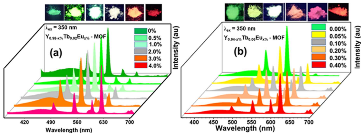
Figure 3. (a) PL emission spectra ( \lambda_{\text{ex}} = 350 \text{ nm} ) of bipyridine containing \text{Y}_{0.98-x}\text{Tb}_{0.02}\text{Eu}_x\% samples with different Eu 3+ concentrations ( 0 < x < 4.0 ) (b) PL emission spectra ( \lambda_{\text{ex}} = 350 \text{ nm} ) of 1, 10 phenanthroline containing \text{Y}_{0.94-x}\text{Tb}_{0.06}\text{Eu}_x\% samples with different Eu 3+ concentrations ( 0 < x < 0.4 ). Note that white light emission was observed at 2% and 0.1% for the bpy and phen compounds, respectively.
