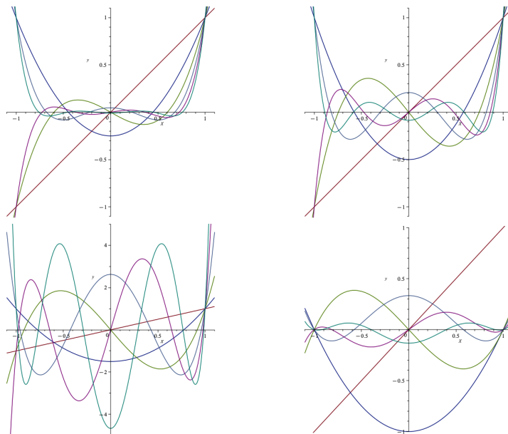
Figure 1: According to Proposition 1 , the first six polynomials R_1(x), \dots, R_6(x) have interlaced roots. Top left display: a = \frac{1}{4} ; top right: a = \frac{1}{2} , these are the Chebychev polynomials; bottom left: a = \frac{3}{2} ; bottom right: a = +\infty .
