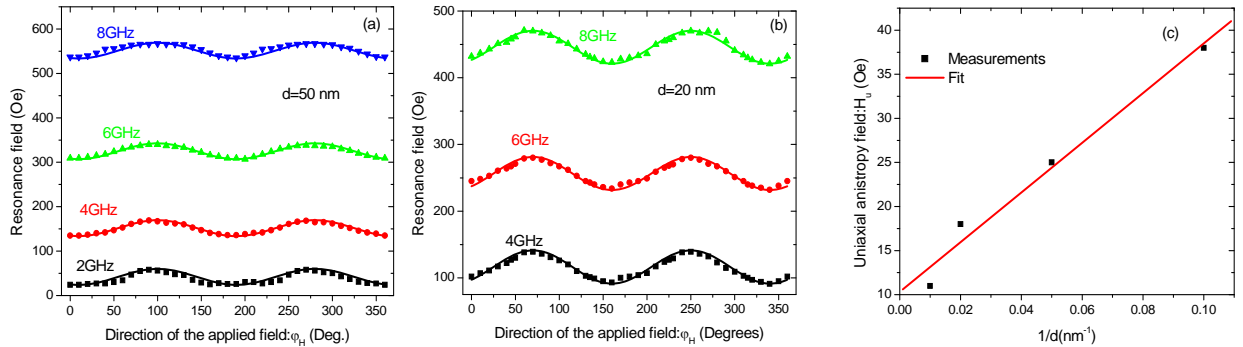
Figure 4: Angular dependence of the resonance field of (a) 50 nm and (b) 20 nm thick Co 2 FeAl thin films. The solid lines refer to the fit using the above mentioned models. (c) Thickness dependence of the uniaxial ( H_u ) extracted from the fit of MS-FMR measurements. The solid lines are the linear fits.
