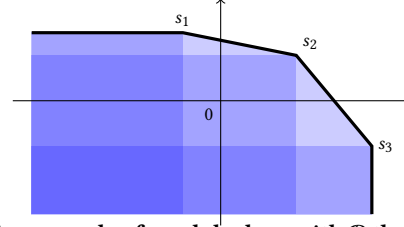
Figure 1: An example of a polyhedron with \mathcal{P} the convex hull of the s_i + \mathbb{R}_{<0}^2 's in \mathbb{R}^2 .
