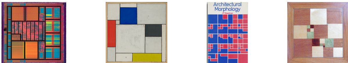
Figure 1: a) VLSI are rectangulations playing an important role for integrated circuits. b) The artwork Composition décentralisée , 1924, by Theo van Doesburg (1883–1931). c) A book on the geometry of building plans [19]. Its cover is not a rectangulation according to our definition (as it contains instances of 4 rectangles meeting in a point). d) This solution to Tutte’s famous “Squaring the square” is a rectangulation.
