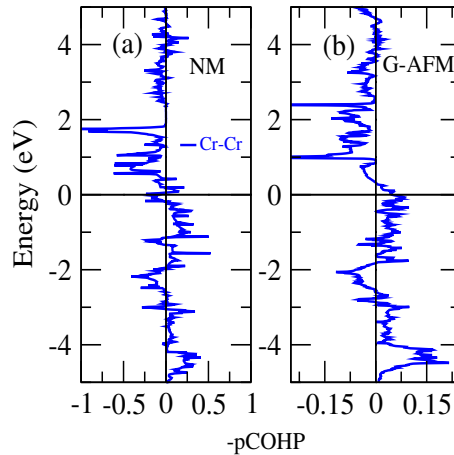
FIG. 4: COHP bonding analysis of Cr-Cr bonds in \text{ThCrAsN} for (a) NM and (b) GAFM phase
