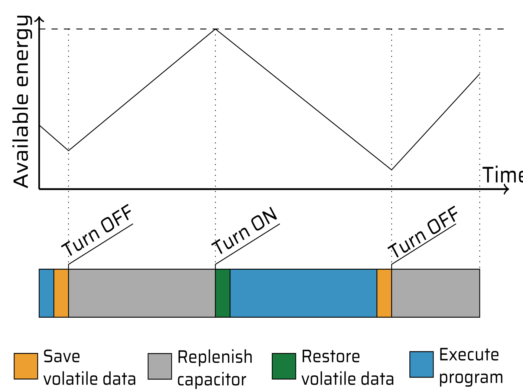
Figure 2 Intermittent execution
