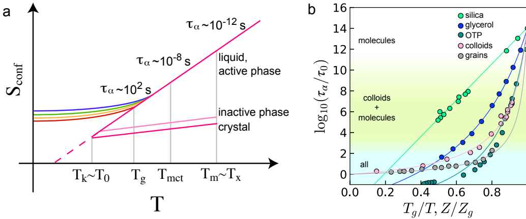
Figure 2. Roadmaps to the glass transition: the configurational entropy and the “Angell plot”.
