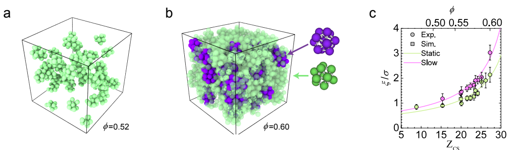
Figure 9. The change in structure in a colloidal glassformer and growth of structural and dynamical lengthscales. Analysis of super-resolution images of small colloidal particles, allowing deeper supercooling than otherwise possible. (a,b) Renderings of locally favoured structures, 10-membered defective icosahedra (green) and 13-membered full icosahedra (purple) for volume fractions of \phi = 0.52 (weakly supercooled) and \phi = 0.60 (deeply supercooled) respectively. (c) Static and dynamic lengthscales \xi_{\text{Static}} and \xi_{\text{Slow}} obtained for defective icosahedra and slow moving particles respectively. Solid lines are fits inspired by RFOT. Reproduced from [47].
