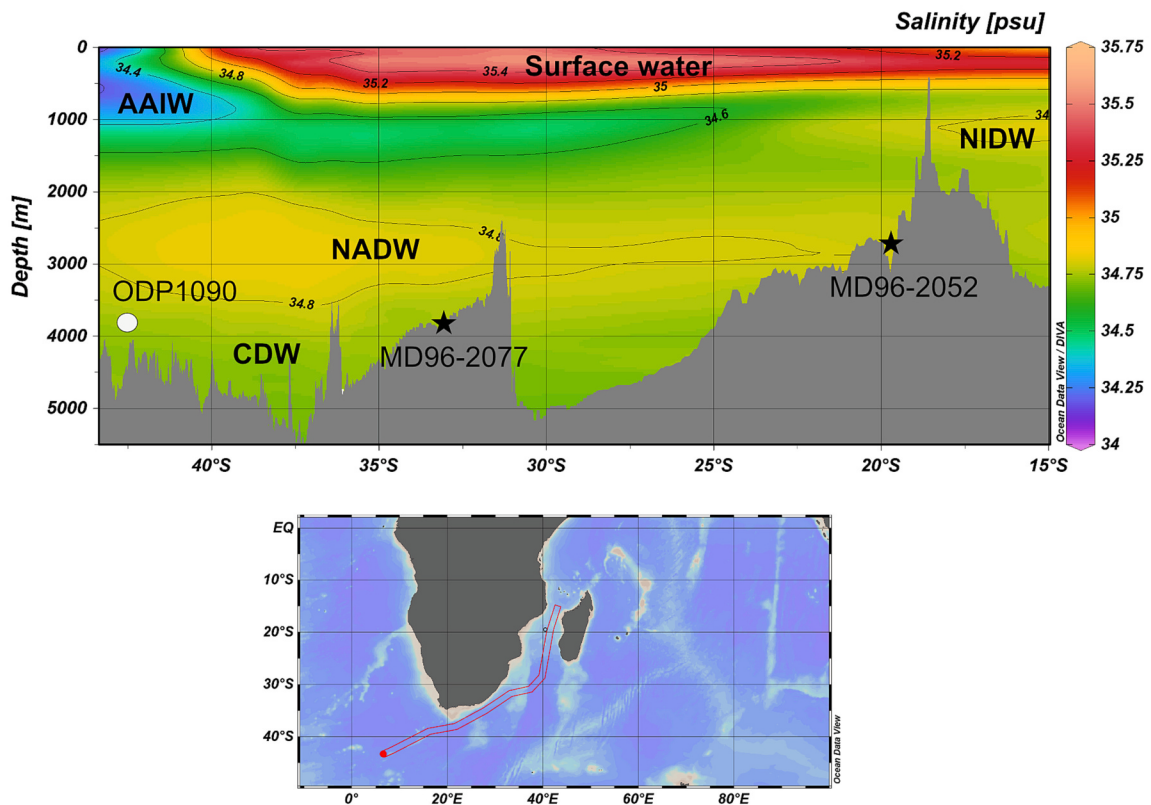
Fig. 1. a) Simplified modern ocean circulation of the study area with the core locations of this study (black stars): MD96-2077 (33°10.1'S, 31°14.8'E, 3781 m water depth), and core MD96-2052 (19°52.7'S, 41°49.9'E, 2627 m water depth); and previous studies cores (white dots): core Agulhas Plateau (AP) composite site (41°19.9'S, 25°49.7'E, 2907 m water depth) (Ziegler et al., 2013; Starr et al., 2021), core MD84-527 (43°49'3S, 51°19'E, 3262 m water depth) (Pichon et al., 1992), core ODP1090 (42°54.82'S, 8°53.98'E, 3702 m water depth) (Hodell et al., 2003) and core SK129-CR2 (3°N, 76°E, 3800 m water depth) (Piotrowski et al., 2009). The colored arrows depict modern flow paths of different water masses: North Atlantic Deep Water (NADW, blue), Circumpolar Deep Water (CDW, purple), and Antarctic Bottom Water (AABW, dark brown). b) SW-NE salinity transect along latitude showing the major water masses: NADW, CDW, AAIW (Antarctic Intermediate Water), NIDW (North Indian Deep Water) and surface water. Symbols as for a). Figures are created with the software Ocean Data View (ODV) (Schlitzer, 2015). (For interpretation of the references to color in this figure legend, the reader is referred to the web version of this article.)
