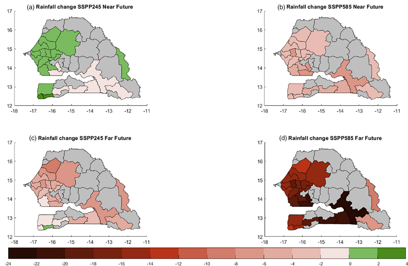
FIGURE 9 Change future (near future and far future) minus present (2000–2013) during JJAS period in % simulated by ensemble mean of CMIP6 models bias-corrected under the SSP2-45 and SSP5-85 scenarios [Colour figure can be viewed at wileyonlinelibrary.com ]
