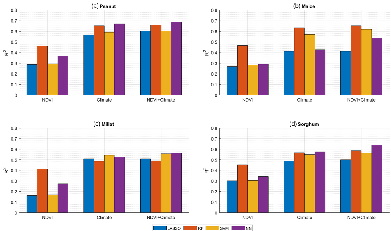
FIGURE 2 The models performance (mean predicted R^2 ) of four regression models using three combination of inputs (NDVI only, Climate only and NDVI+Climate) averaged over the rainy season (June–September) for peanut (a), maize (b), millet (c) and sorghum (d) [Colour figure can be viewed at wileyonlinelibrary.com ]
