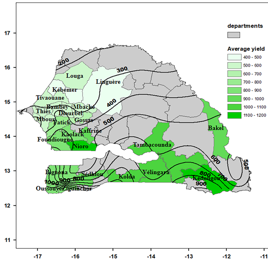
FIGURE 1 Map of studied area. Selected departments with crop yield data (in green). The department in grey were not used in this study (no crop yield data). Shaded values represent the 2000–2013 mean of crop yields of maize, millet, sorghum and peanut ( \text{kg}\cdot\text{ha}^{-1} ). Contour lines represent the annual rainfall ( \text{mm}\cdot\text{year}^{-1} ) based on the rain gauge stations network of the National Agency for Civil Aviation and Meteorology during summer (June–September) from 1991 to 2005 [Colour figure can be viewed at wileyonlinelibrary.com ]
