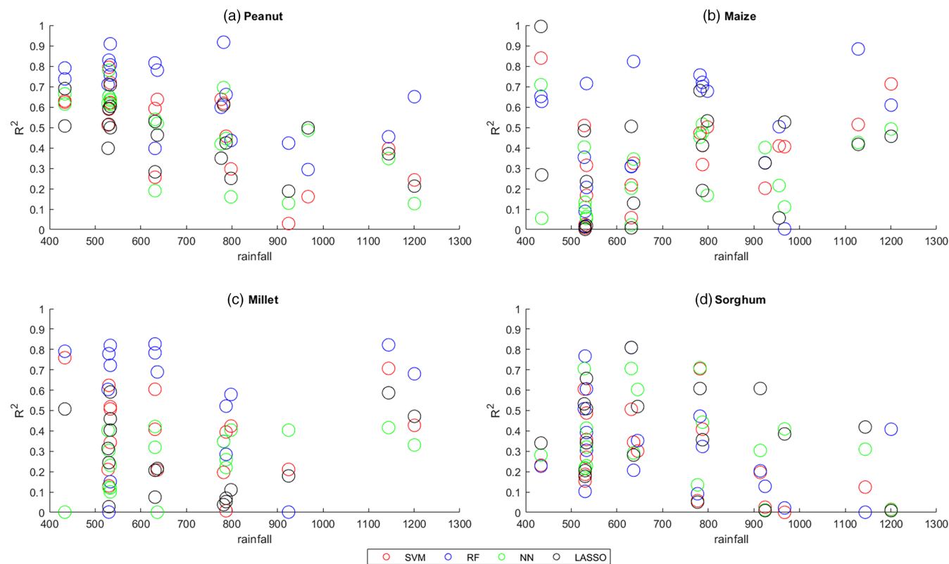
FIGURE 5 Predicted R^2 of the regression models at the department level (one colour per model) and June to September accumulated rainfall ( \text{mm}\cdot\text{season}^{-1} ). As for Figure 4, the statistical models use NDVI+Climate combination from June to September to predict yield of peanut (a), maize (b), millet (c) and sorghum (d). We fit/test the four models (NN, LASSO, RF and SVM) using data from all departments and years together. We thus have four mean predictions for each department and each year. We then extract the predictions for one department and calculate R^2 separately for each of the four methods [Colour figure can be viewed at wileyonlinelibrary.com ]
