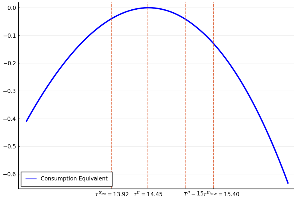
Figure 6: Welfare with transitions and a fixed-point initial distribution, computed as a function of the tax rate.
