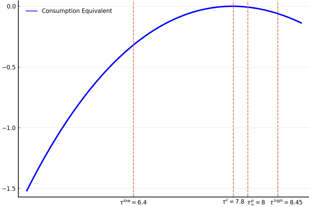
Figure 1: Welfare with transitions and fixed-point initial distribution computed as a function of the tax rate. See the text for the definitions of other tax rates.
