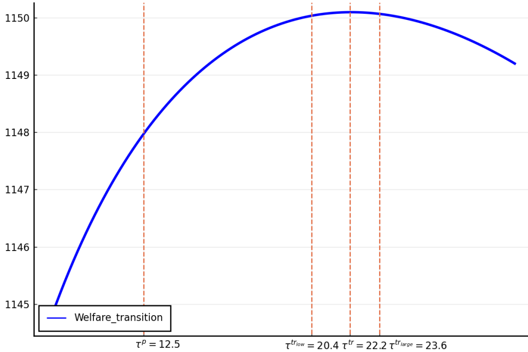
Figure 4: Welfare with transition approach and fixed-point initial distribution computed as a function of the labor tax rate.
