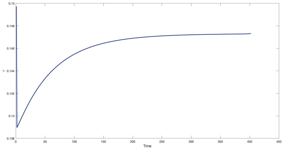
Figure 7: Dynamic of the tax after a reoptimization shock when the curvature of v is \vartheta = 65\% .
