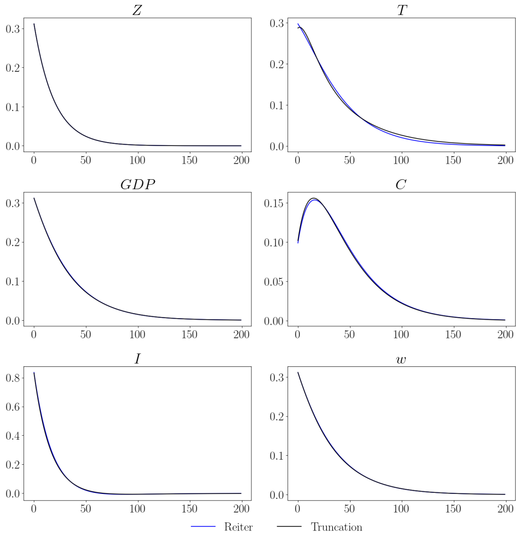
Figure 5: Simulated IRFs after a TFP shock simulated using the truncation approach and Reiter method. See the text for the details of the implementations.
