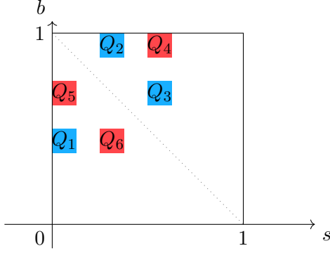
Figure 1: The squares Q_1, \dots, Q_6 appearing in the proof of Theorem 2.
