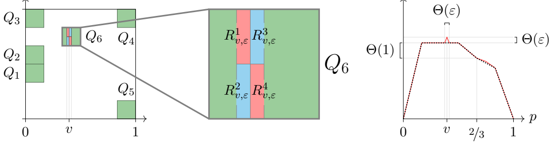
Figure 2: Left/center: The six squares Q_1, \dots, Q_6 (in green) are the support of the base density f , and the four rectangles R_{v,\varepsilon}^1, \dots, R_{v,\varepsilon}^4 (in red and blue) inside Q_6 are the regions where the density is perturbed with g_{v,\varepsilon} . Right: The corresponding qualitative plots of p \mapsto \mathbb{E}[\text{GFT}(p, S, B)] (black, dotted) and p \mapsto \mathbb{E}^{v,\varepsilon}[\text{GFT}(p, S, B)] (red, solid).
