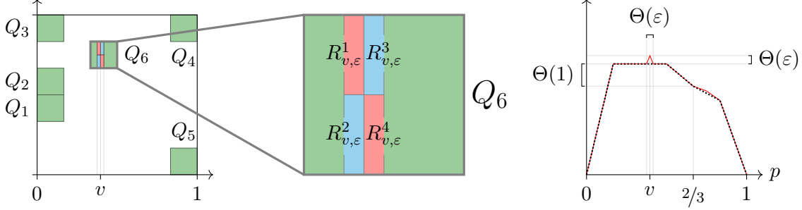
Figure 2: Left/center: The six squares Q_1, \dots, Q_6 (in green) are the support of the base density f , and the four rectangles R_{v,\epsilon}^1, \dots, R_{v,\epsilon}^4 (in red and blue) inside Q_6 are the regions where the density is perturbed with g_{v,\epsilon} . Right: The corresponding qualitative plots of p \mapsto \mathbb{E}[\text{GFT}(p, S, B)] (black, dotted) and p \mapsto \mathbb{E}^{v,\epsilon}[\text{GFT}(p, S, B)] (red, solid).
