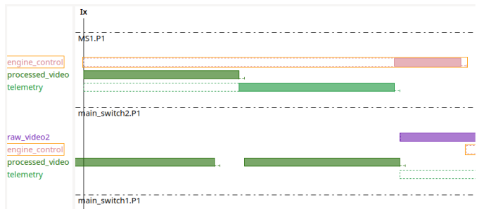
Fig. 7. Gantt charts for the engine_control data stream in RTaW-Pegase
