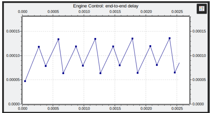
Fig. 6. End-to-end delay of the engine_control stream without using the Time Aware Shaper in NeSTiNg
