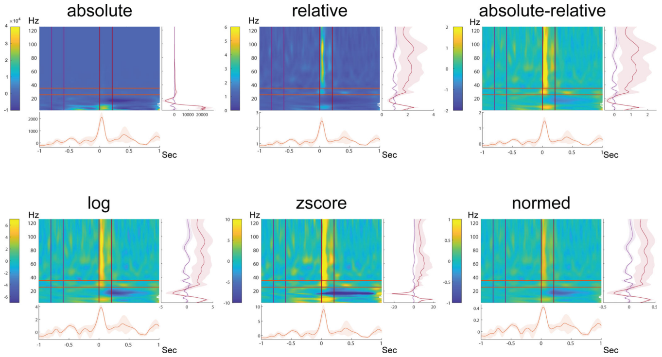
Figure 13. Baseline correction and time frequency representation. The same time-frequency representation of power is depicted with different baselining methods computed from -1 sec to -0.5 s. Within a frequency range (orange) and two time ranges of interest (purple and red), the mean and the mean-absolute-deviation are depicted at the bottom and on the side. The choice of the baselining method enhances/reduces the visibility of particular features in the data (for instance the 1/f effect, see sections 4.2.3.3 and 4.2.3.4.1).
