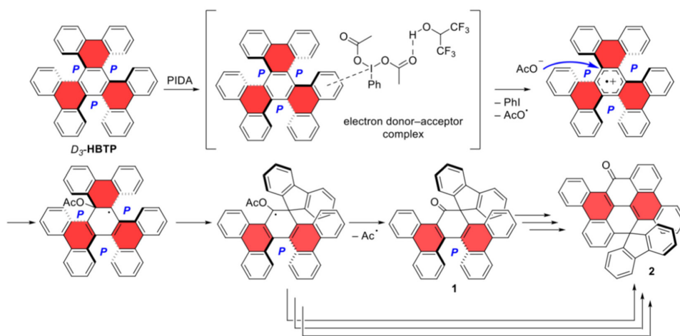
Scheme 2 Mechanistic hypotheses.
