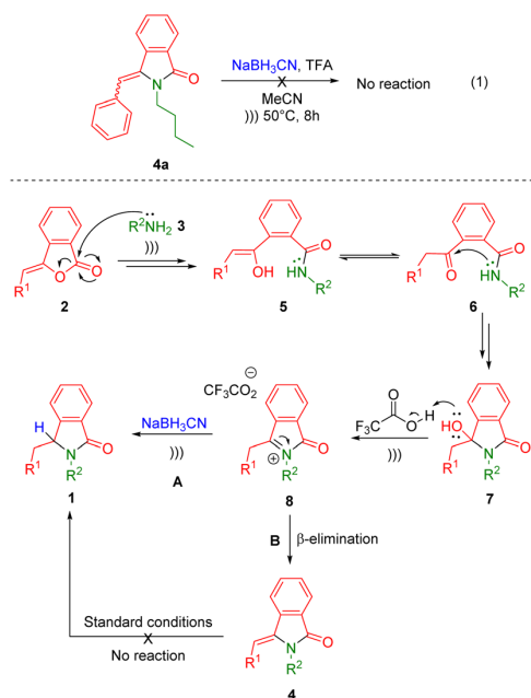
Scheme 2 Proposed reaction mechanism.
