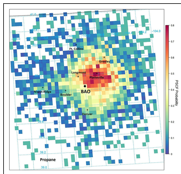
Figure 3. Potential Source Contribution Function results for propane greater than the median for 2007–2016 (data for all seasons; n = 2,520 ) in flasks collected during daytime hours at Boulder Atmospheric Observatory (black dot). DOI: https://doi.org/10.1525/elementa.2020.00136.f3
