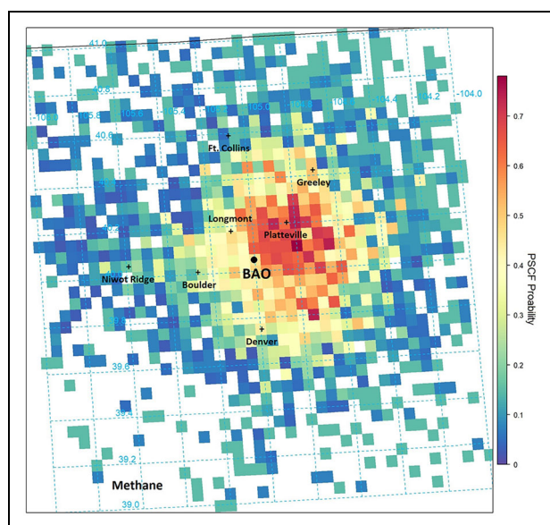
Figure 2. Potential Source Contribution Function results for methane greater than the median for 2007–2016 (data for all seasons; n = 2,728 ) in flasks collected during daytime hours at Boulder Atmospheric Observatory (black dot). DOI: https://doi.org/10.1525/elementa.2020.00136.f2
