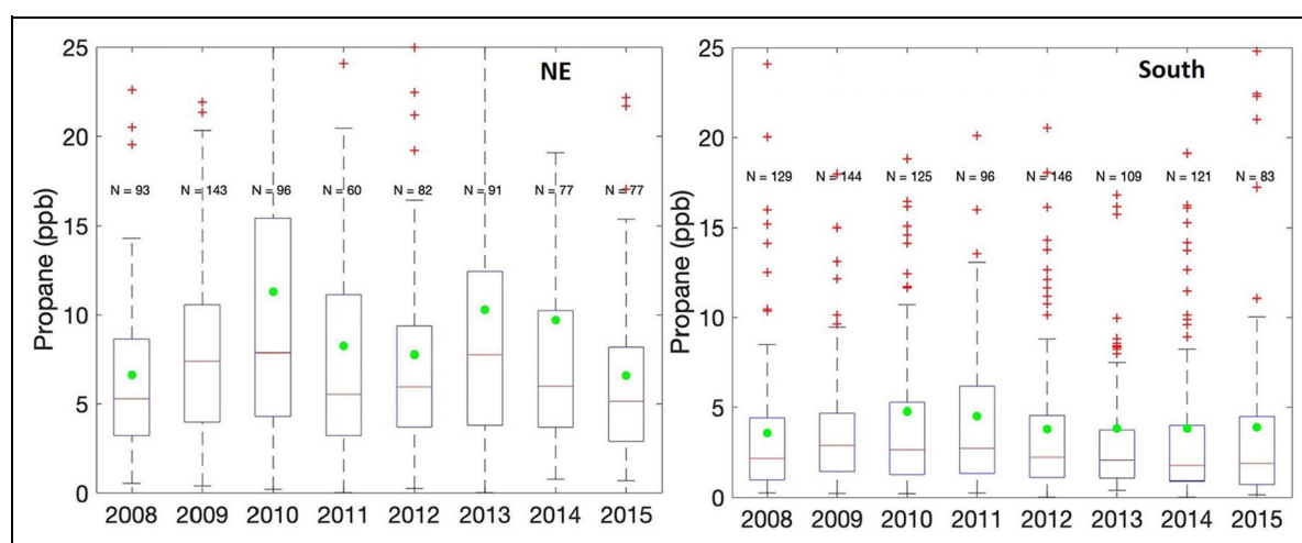
Figure 6. Annual distribution of propane mole fractions at Boulder Atmospheric Observatory for each year for daytime samples collected when winds at the tower were from the northeast (NE) quadrant (left panel) and for daytime samples collected when winds at the tower were from the south (right panel). The horizontal red line in each box is the median, the box bottom and top are the 25th and 75th percentiles, the vertical bars indicate the 5th and 95th percentiles, the red pluses values >95th percentile, and the green dots are the mean (in 2009, the mean was above the upper limit of the y-axis; very high individual samples for the NE quadrant are not encompassed within the 25 ppb y-axis limit where samples exceeded 50 ppb [highest value >100 ppb]). Annual statistics were calculated using daytime individual flask samples ( N ) including all 12 months of the year. DOI: https://doi.org/10.1525/elementa.2020.00136.f6
