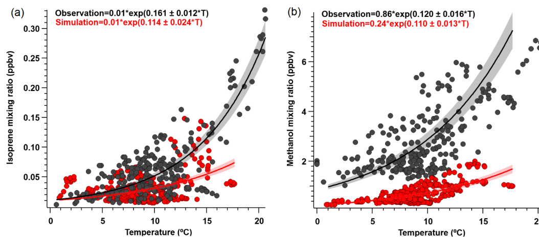
Figure 6. Ambient (a) isoprene and (b) methanol mixing ratio (ppbv) versus temperature (°) for daytime values (08:00 to 20:00 LT) where PAR > 400 μmol m -2 s -1 . Solid lines show exponential fits (major axis regression) to observations (black) and modeled (red) outputs, following the exponential temperature activity factor in Eq. (2) (Guenther et al., 2012). Shaded areas represent 95 % confidence intervals; r^2 \geq 0.5 for both species.
