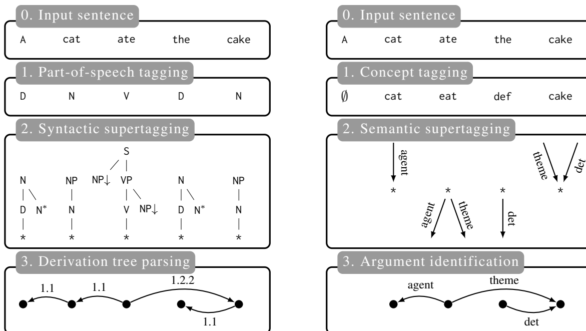
Figure 3: Comparison of a LTAG parsing pipeline and the proposed semantic parsing pipeline. (left) A standard LTAG parsing pipeline. We start with an input sentence, then predict one part-of-speech tag per word. This part-of-speech can be used as feature or to filter the set of possible supertags in the next step. The supertagging step chooses one supertag per word. Finally, in the last step we merge all supertags together. This operation can be synthesised as a derivation tree where arc labels indicate Gorn addresses of substitution and adjunction operations. We refer readers unfamiliar with LTAG parsing to (Kallmeyer, 2010). (right) Our semantic parsing pipeline. We start with an input sentence, then predict at most one concept per word, where \emptyset indicates no concept. The supertagging step assigns one supertag per concept instance ( i.e. , excluding words tagged with \emptyset ). Finally, the argument identification step identifies arguments of predicates using the valency constraints from the supertags.
