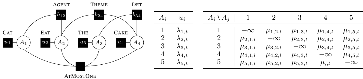
Figure 4: (left) The factor graph used to compute the best alignment of the semantic graph in E steps for the sentence ‘A cat ate the cake’. Each variable corresponds to a concept instance in the semantic graph and has an associated unary factor. For each argument of a concept instance, we add a binary factor between between the concept instance and its argument’s instance. (center) Weights of an unary factor given the value of its corresponding variable. We denote t the concept corresponding to that factor (displayed above unary factors). (right) Weights of a binary factor b_{ij} , where the concept instance represented by A_j is an argument of the concept instance represented by A_i in the semantic graph. We denote l the label of the argument (displayed above binary factors).
