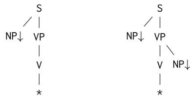
Figure 2: Two supertag examples from an LTAG. (left) Supertag associated with an intransitive verb. The substitution site \text{NP}\downarrow indicates the position of the subject. (right) Supertag associated with a transitive verb. The supplementary substitution site on the right indicates the position of the object of the verbal phrase.
