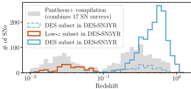
Figure 3. Histogram showing the redshift distribution of the DES-SN5YR sample, with new DES SNe in blue and our low- z sample in red. For comparison, the distribution of redshifts in the existing Pantheon+ sample is shown in gray (D. Brout et al. 2022a), which also includes the DES SNe from the DES-SN3YR analysis (blue dashed line). The 5 yr DES sample contains \sim 4\times more SNe above z \sim 0.4 than the Pantheon+ compilation.
