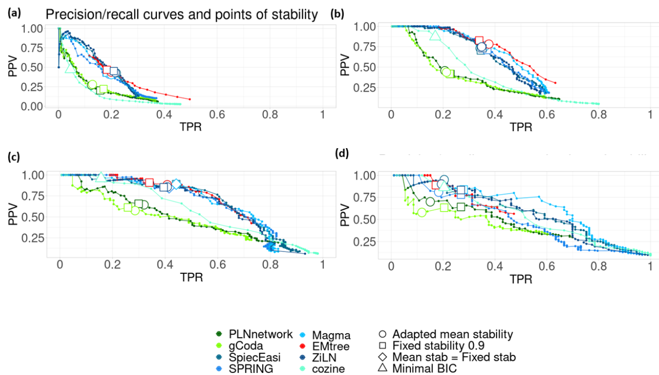
Supplementary Figure S12: Same as Fig. S11 but for size n = 100 .
