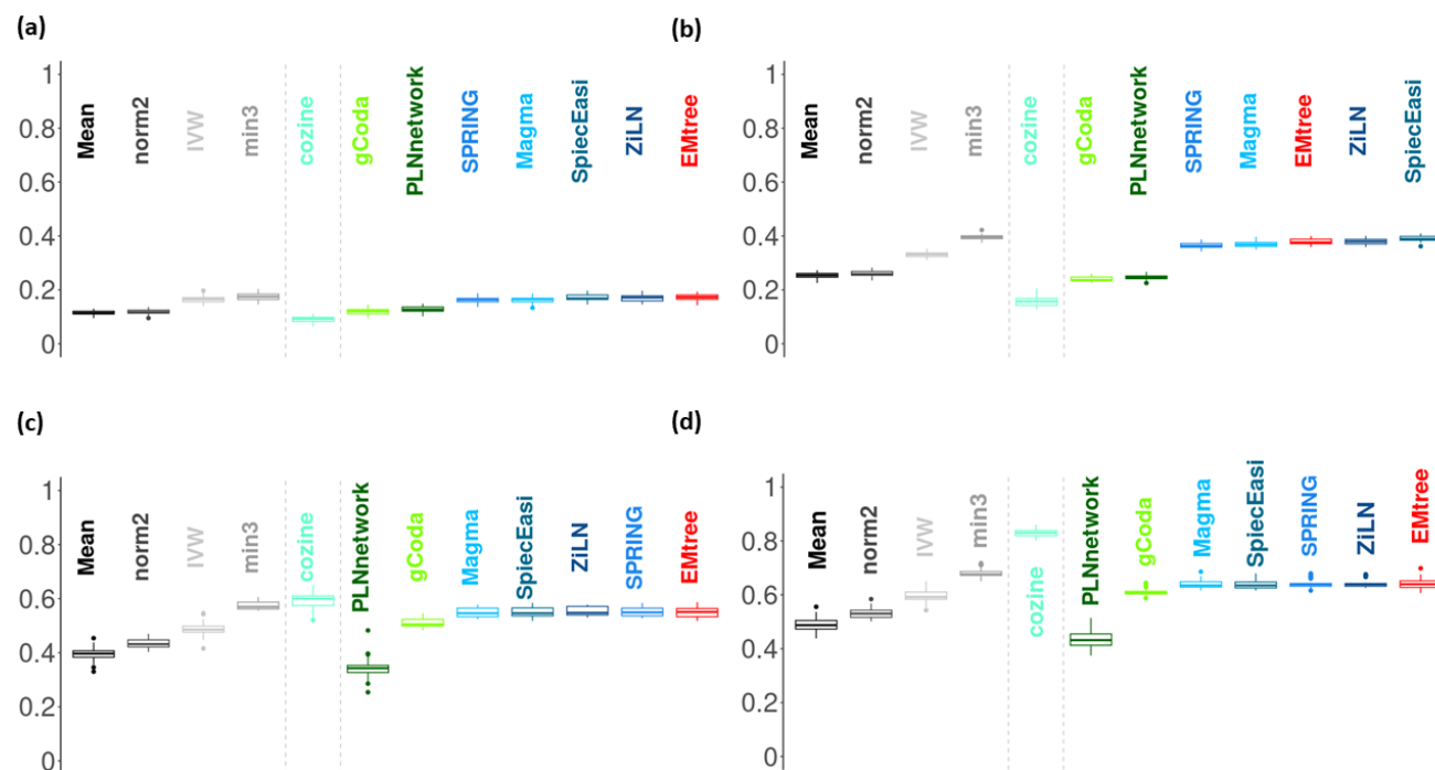
Supplementary Figure S6: Compared precision (PPV) of inference methods and OneNet-* variants when including all 7 methods in the set of methods, for different samples sizes: (a) n = 50 (b) n = 100 (c) n = 500 (d) n = 1000
