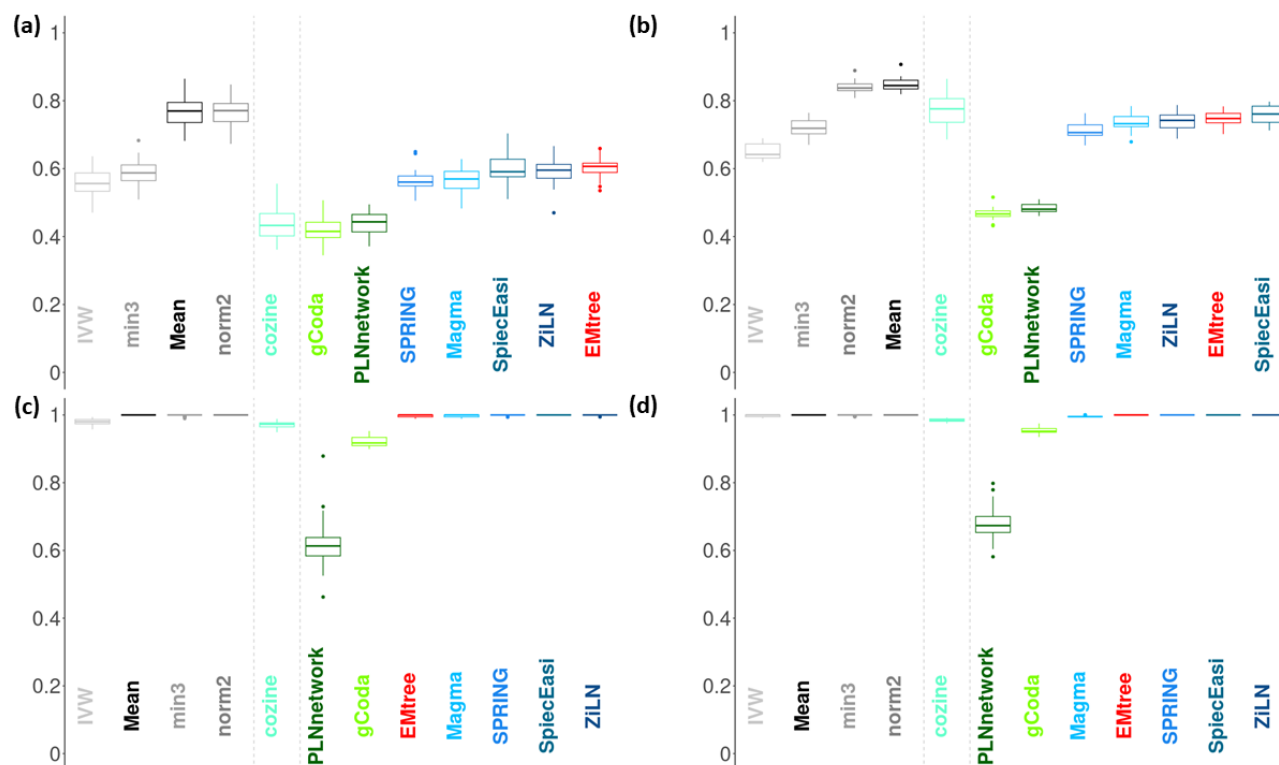
Supplementary Figure S6: Compared precision (PPV) of inference methods and OneNet-* variants when including all 7 methods in the set of methods, for different samples sizes: (a) n = 50 (b) n = 100 (c) n = 500 (d) n = 1000
