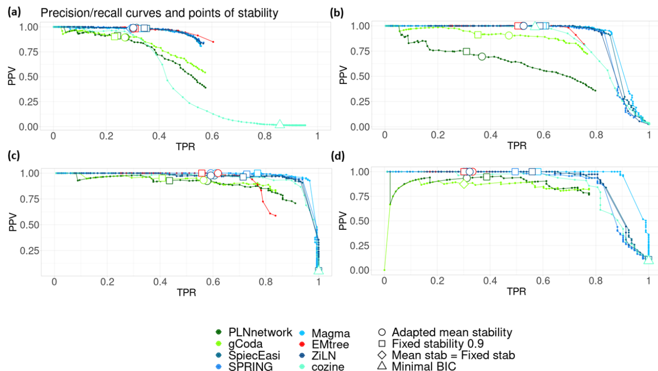
Supplementary Figure S11: Precision - recall curves of each method and TPR/PPV compromise chosen by stability, mean stability and BIC (see figure 3 for details) when n = 500 after filtering the dataset to keep only species with prevalence higher than a given threshold: (a) 0.20 (b) 0.50 (c) 0.8 (d) 0.9
