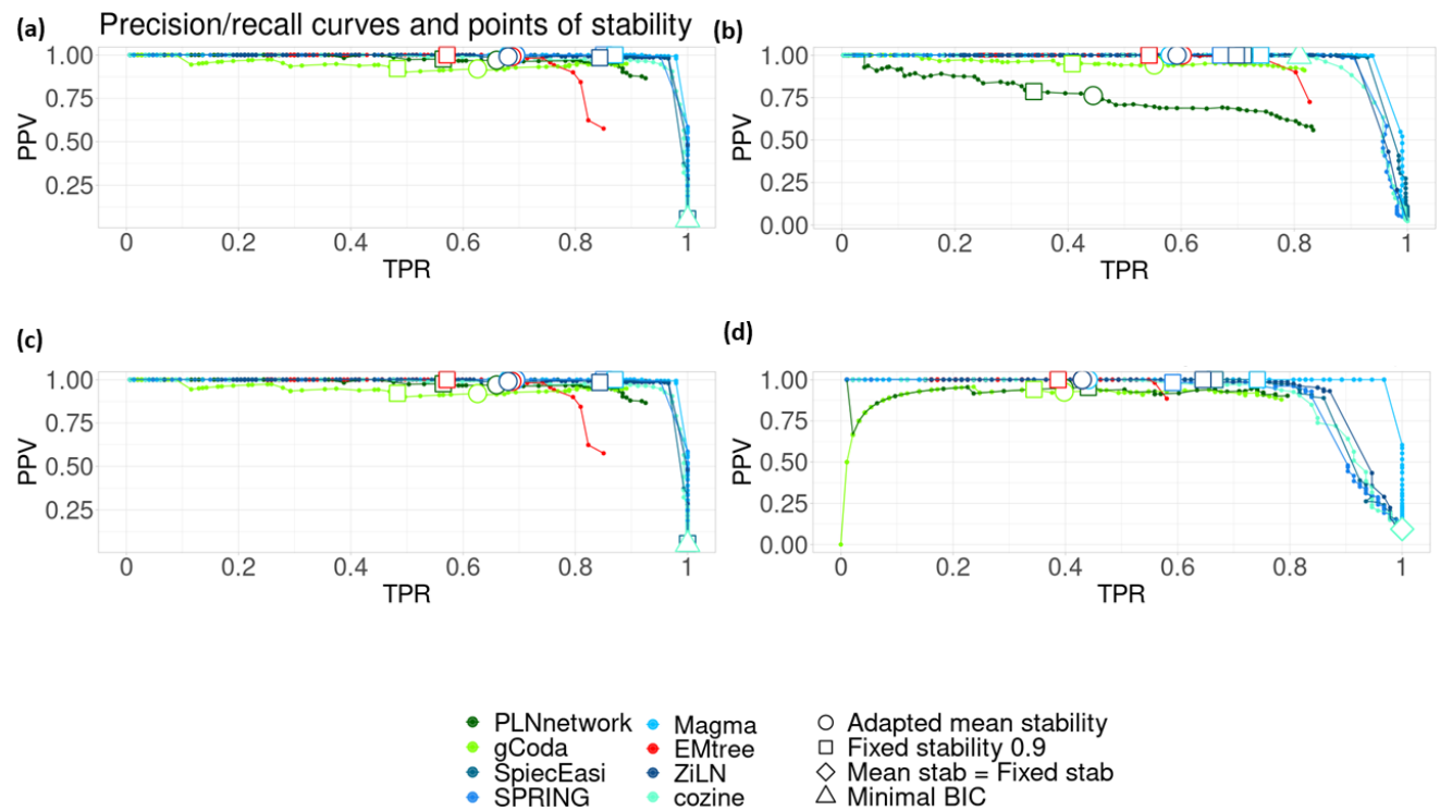
Supplementary Figure S13: Same as Fig. S11 but for size n = 1000 .
