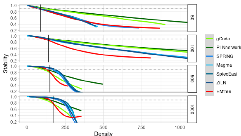
Supplementary Figure S3: Stability - Density curves of the edge set E^\lambda(0.90) according to the sample size and inference method. Each point in the curve corresponds to a different value of \lambda .
