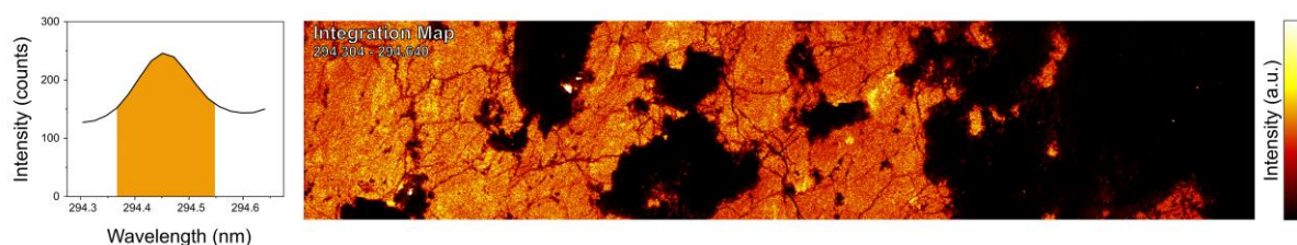
Figure 6: a) The mean spectrum of the dataset between 294.3 and 294.65 nm and, b) , nm and the integration map over the salme spectral range.
