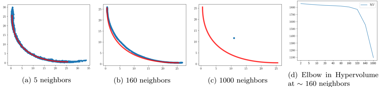
Figure 4: Convex Pareto front estimated through KNN average.
