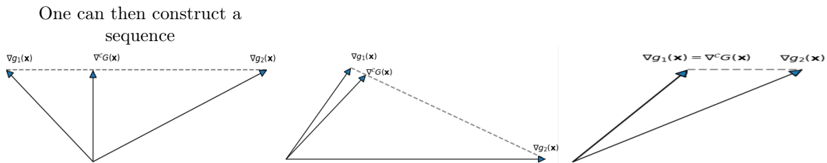
Figure 1: Examples of Calculation of Direction of Descent \nabla_x^C \{G\}(\mathbf{x}) for two objectives.
