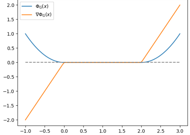
(b) g_1(\mathbf{x}) = (x - 2)^2 , g_2(\mathbf{x}) = x^2 .
