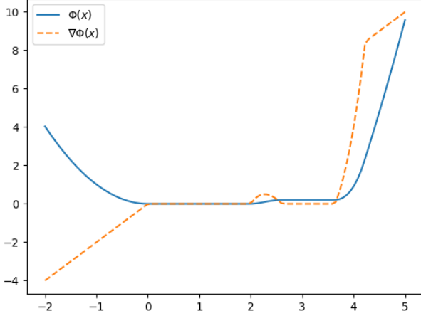
(a) g_1(\mathbf{x}) = (x - 2)^2(x - 3)(x - 4) , g_2(\mathbf{x}) = x^2 .
