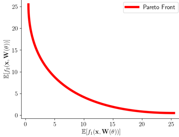
Figure 6: Pareto front for example problem in Objective space
