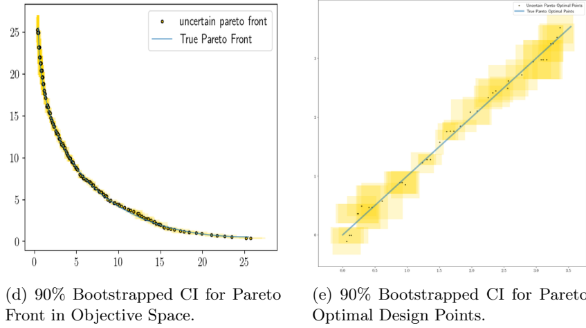
Figure 7: 1000 samples, \varepsilon_0 = .9 , \lambda_0 = 1 , and \varepsilon_\infty = .15 .
