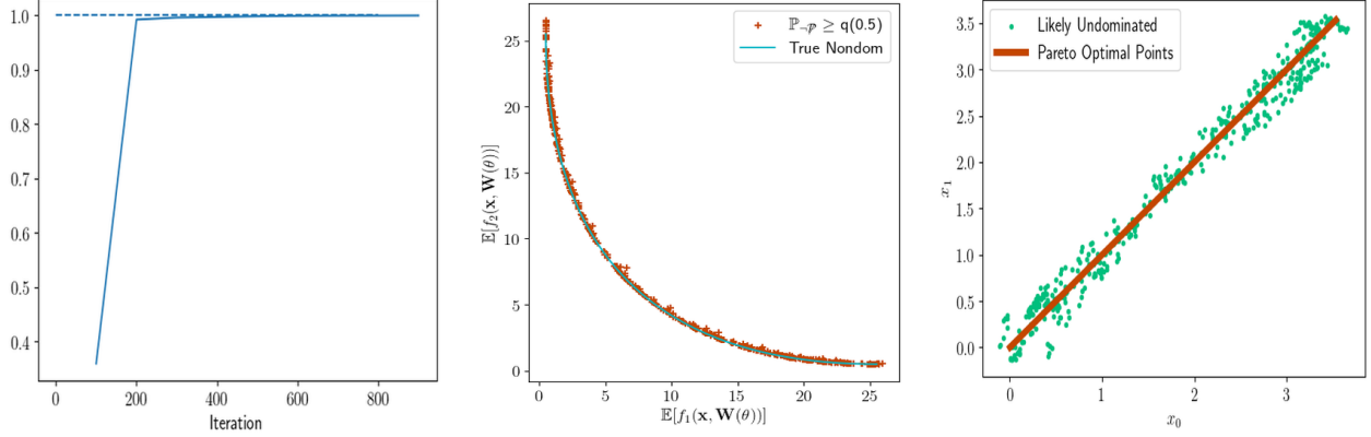
(a) Proportion of the hypervolume captured by the algorithm to the true hypervolume. (b) Probability of Being Undominated Captures Pareto front. (c) Local Mean is Concentrated around True Undominated Points.
