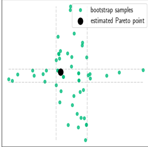
Figure 5: Example estimated Pareto efficient point and corresponding box B_{i,j}
