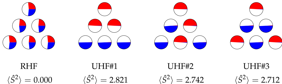
FIG. 3. Mulliken population analysis and the expectation values of \hat{S}^2 for the four HF solutions of the triangular-shaped H_6 cluster (see Table IV). A full half-circle corresponds to an entire spin-up or spin-down electron.
