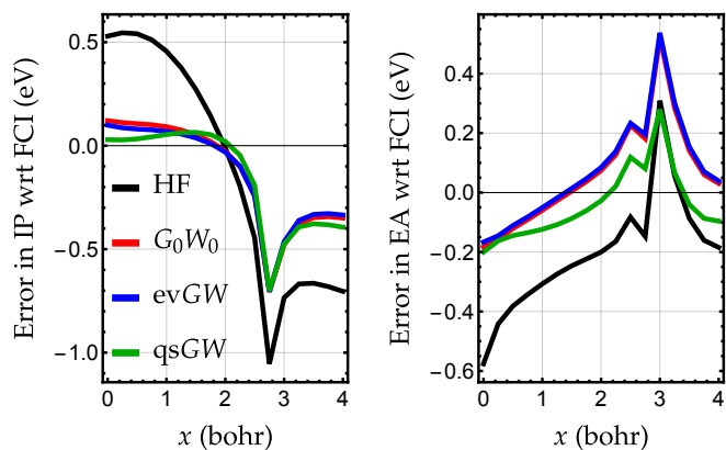
FIG. 2. Error in IP and EA with respect to FCI (in eV) during the insertion reaction of Be into H_2 as a function of x computed at the HF, G_0W_0 , evGW, and qsGW levels.
