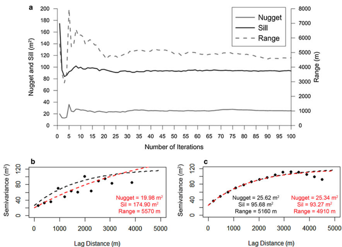
Fig 13. (a) Stabilization of the parameters of the semi-variogram model as a function of the number of iterations of Mer the Glace; and Experimental semi-variogram (black circles) and fitted exponential model of Mer de Glace: the black dashed line stands for the full density topography and the red dashed line stands for the 1st iteration in (b) and for the 50th iteration in (c). The parameters of each semi-variogram model are included.
